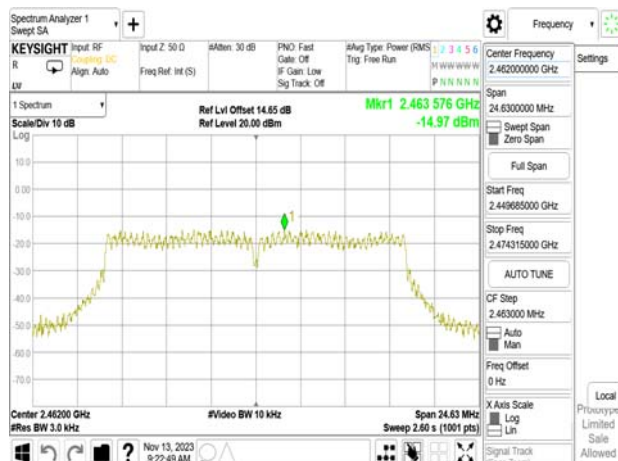
802.11g_20MHz_WLAN2_2462MHz
