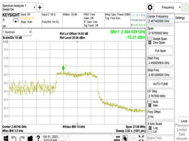
802.11ax_20MHz_WLAN1_2462MHz_RU106_54
