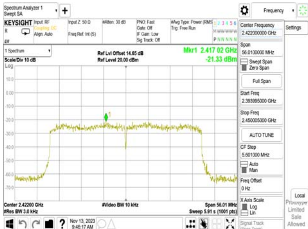
802.11ax_40MHz_WLAN1_2422MHz_RU242_61
