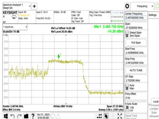
802.11ax_20MHz_WLAN2_2462MHz_RU106_54
