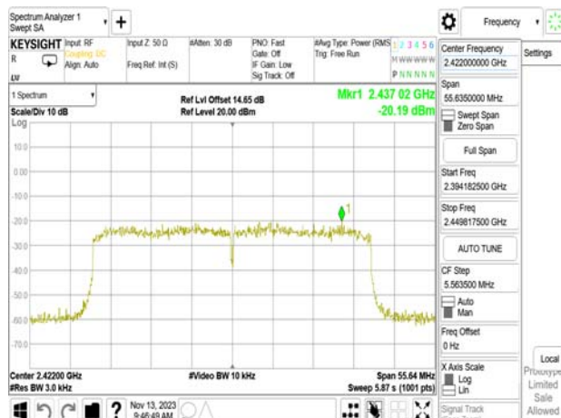
802.11ax_40MHz_WLAN2_2422MHz
