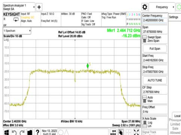
802.11ax_20MHz_WLAN1_2462MHz
