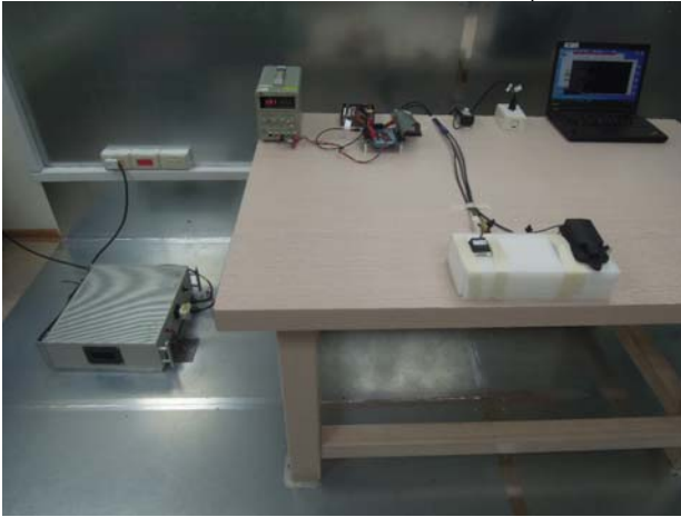
FCC_15_407_WLAN_Conduction_Setup
