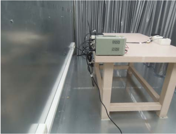
FCC_15_407_WLAN_Conducted_Setup
