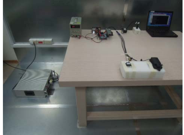
FCC_15_247_WLAN_Conduction_Setup
