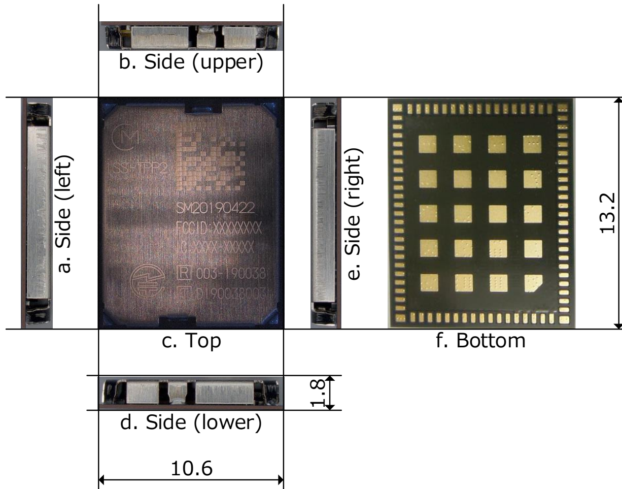
Fig. 1SS, 6D photo (unit: mm)
