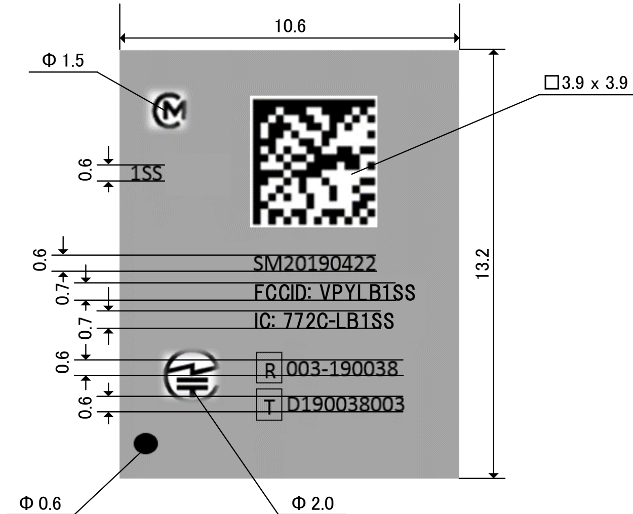
Fig. Dimension (Unit: mm)
