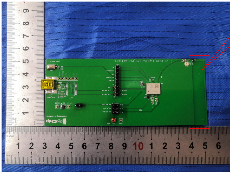
PCB antenna
