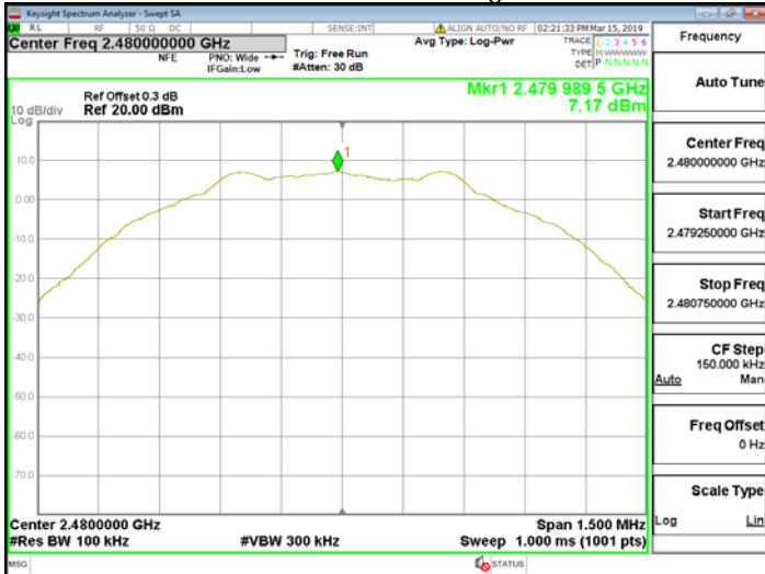
Reference Level_BLE_1M_HighCH39-2480
