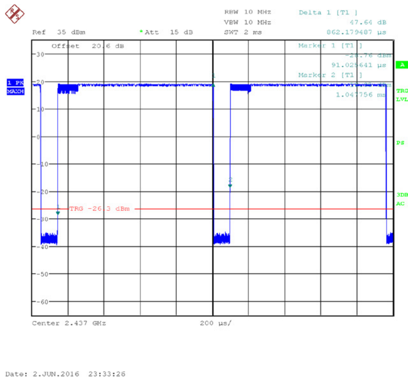
Figure 7.6.2-1: Duty Cycle 802.11b
