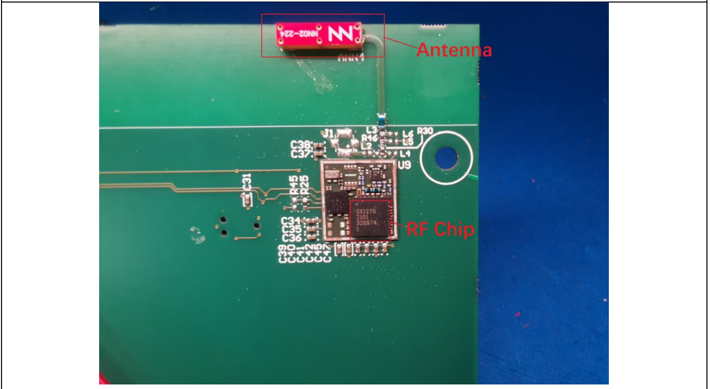
EUT Photo(1)
