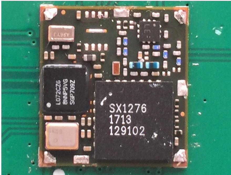
EUT on Test Board-1 View (With PCB Antenna)
