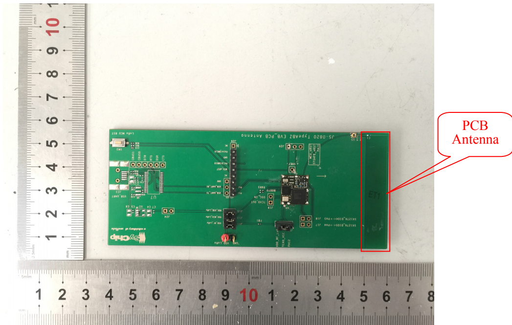
EUT on Test Board-1 View (With PCB Antenna)
