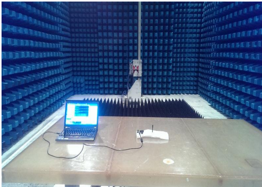
Photograph 2: Set-up for Radiated Emission, above 1GHz
