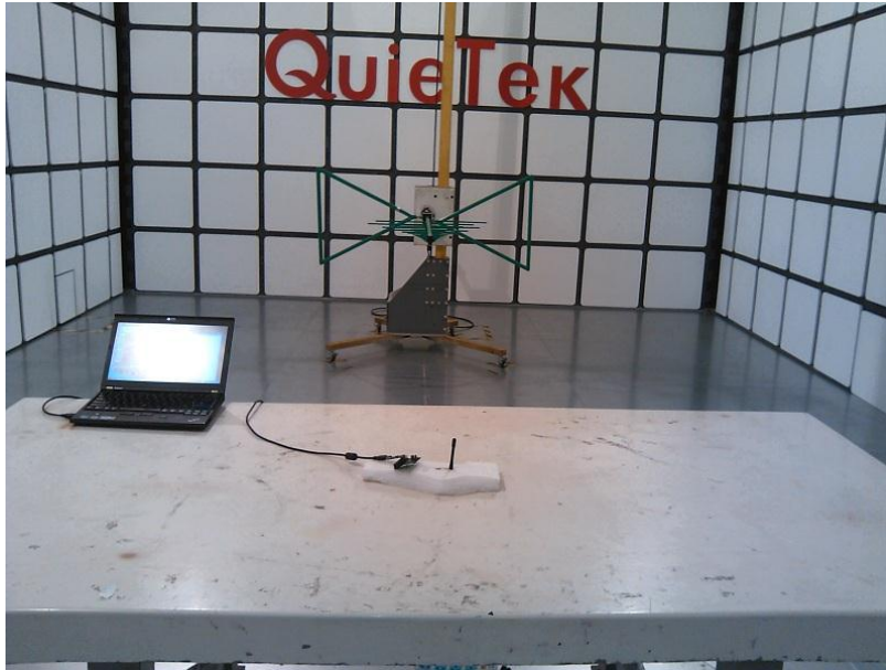
Photograph 1: Set-up for Radiated Emission, 30MHz-1000MHz
