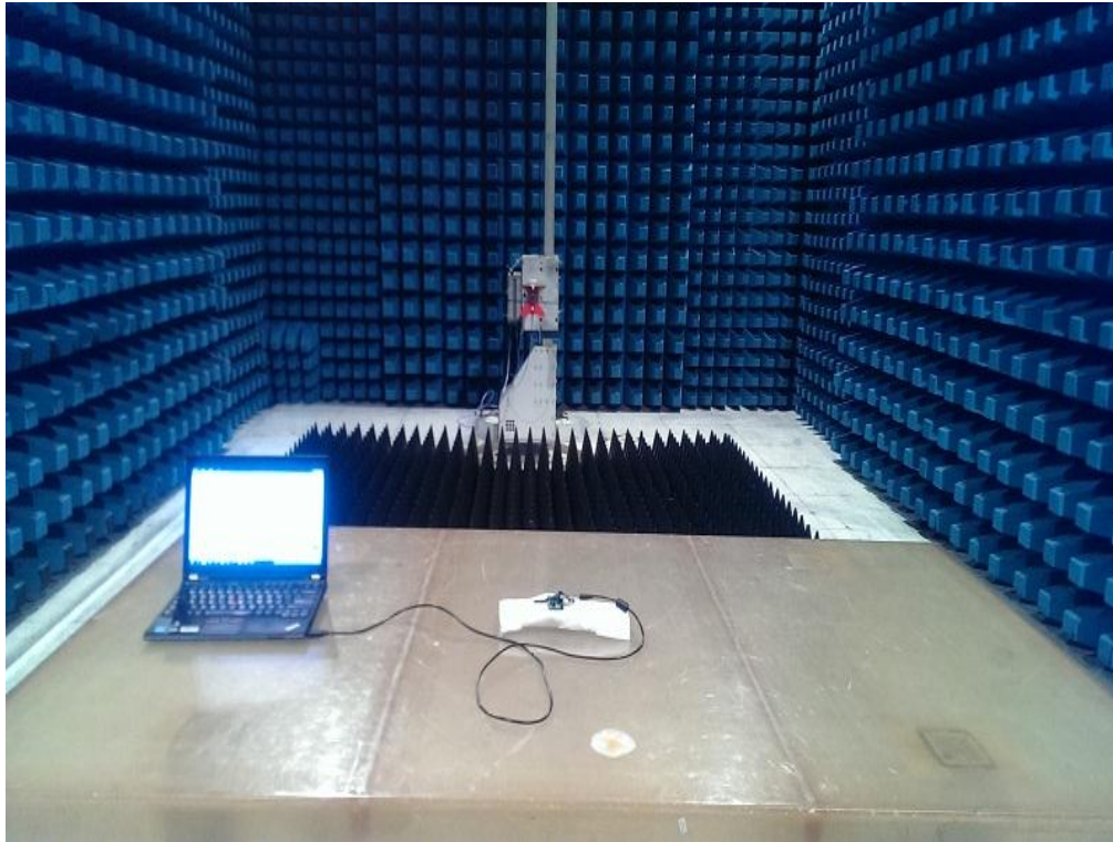
Photograph 2: Set-up for Radiated Emission, above 1GHz
