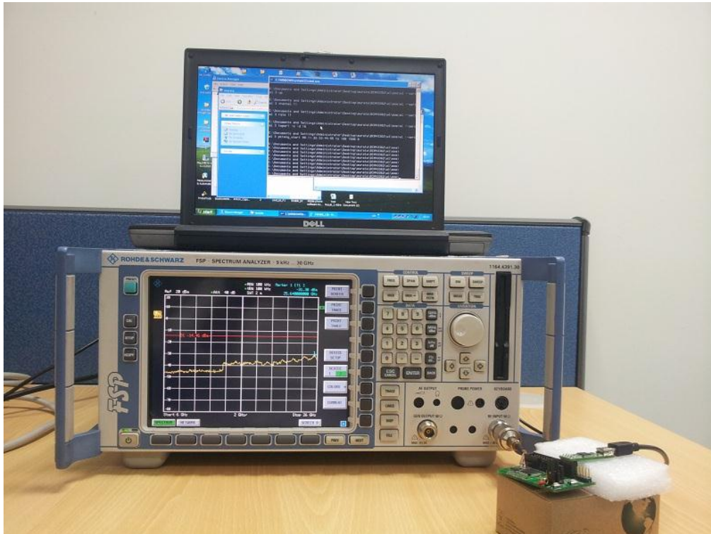
Photograph 3: Set-up for RF Power
