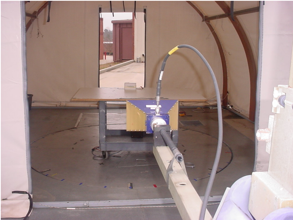
Figure 2: Test Setup – Radiated Emissions – Intentional
