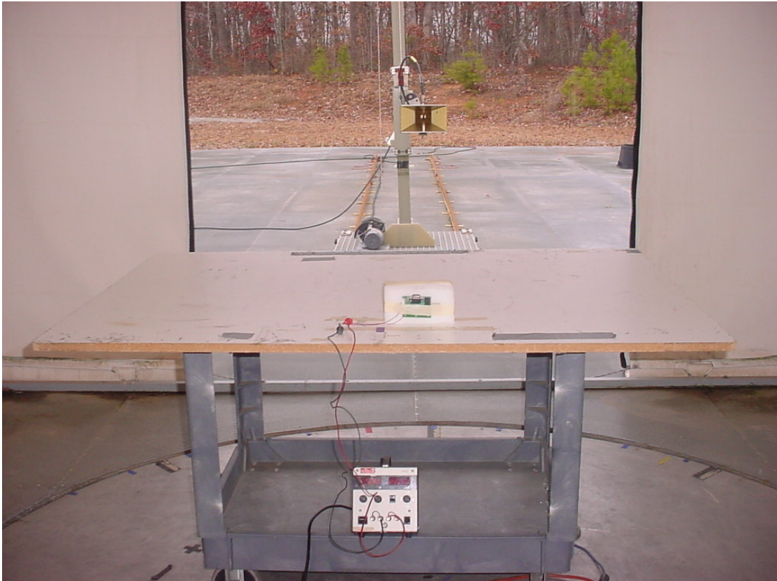
Figure 1: Test Setup – Radiated Emissions – Intentional
