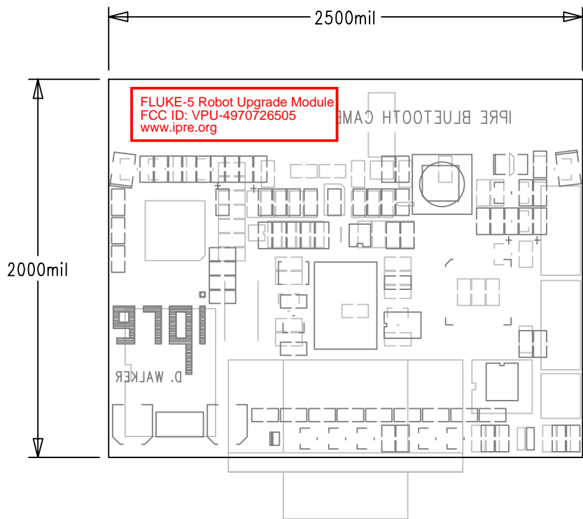
FCC label positioning. The label is 0.9375"x0.3125". It is silkscreened directly on the top of the PCB. There is no case.
