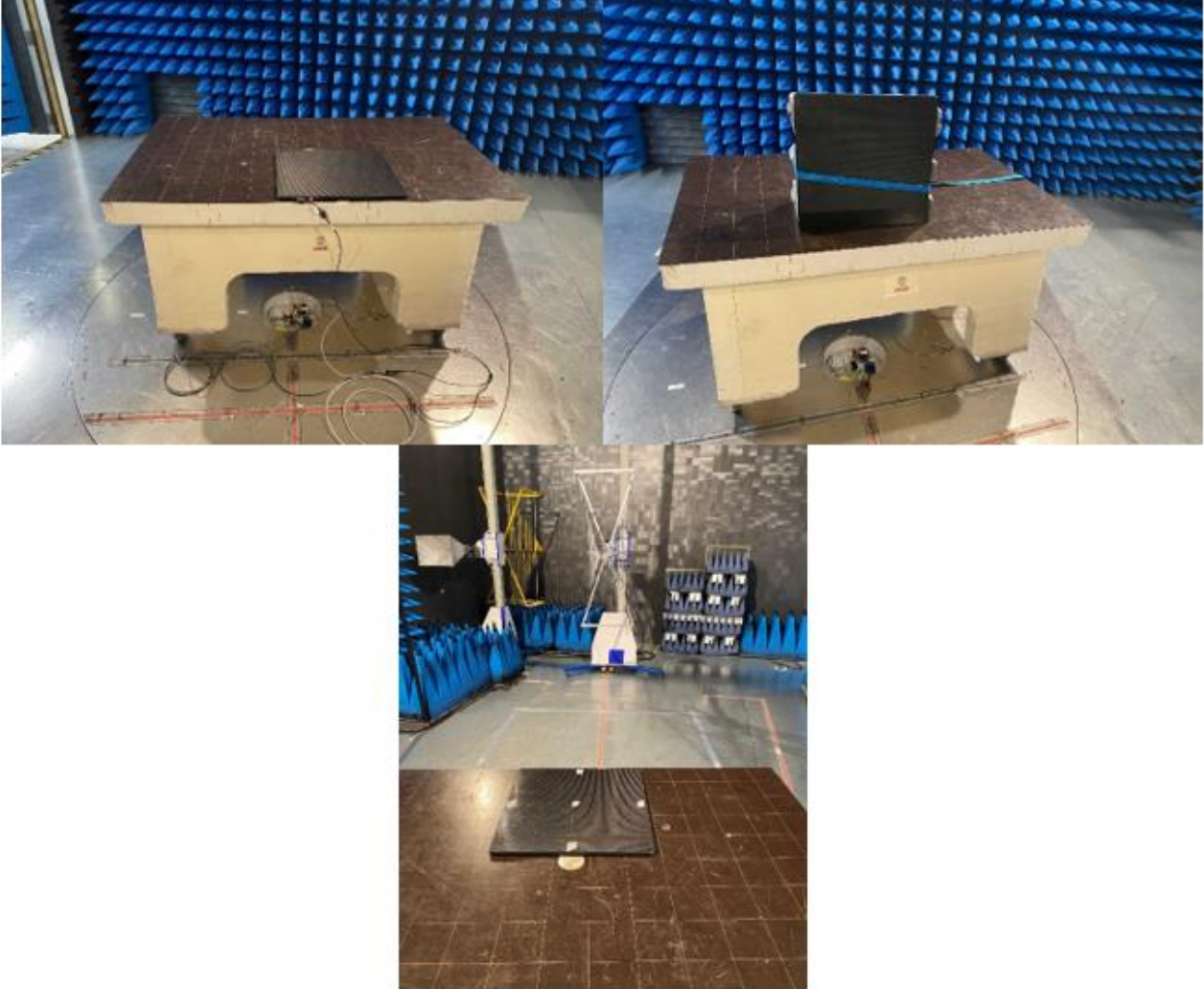
Test setup in anechoic chamber – Frequency <1GHz
