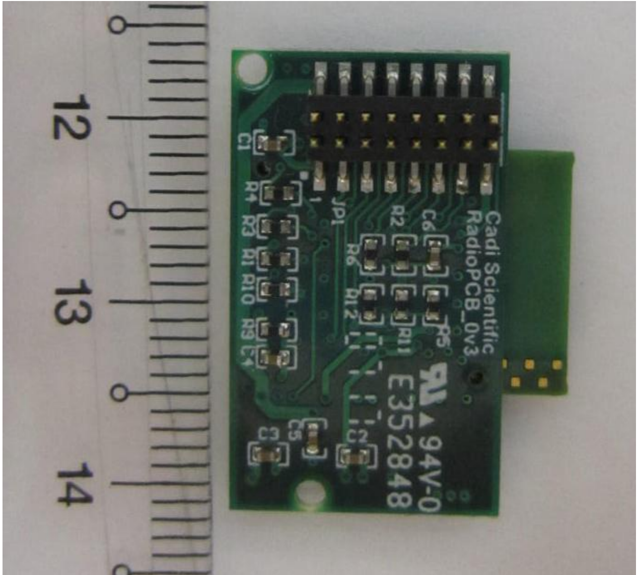
Module Board PCB Trace Side
