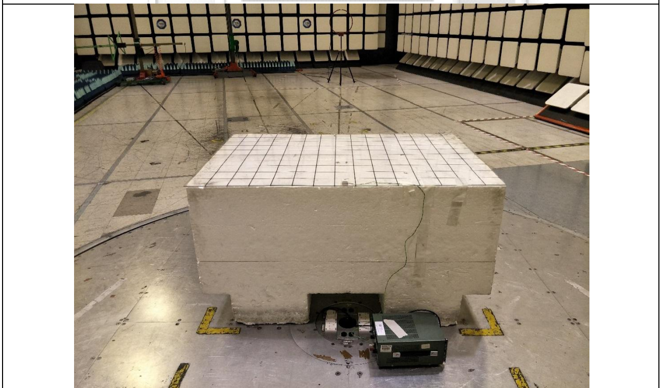
Radiated Emissions Test Setup (Rear View)
