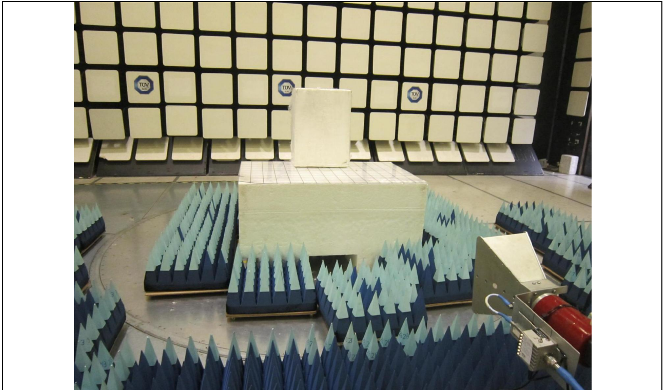
Radiated Emissions Test Setup (Front View)
