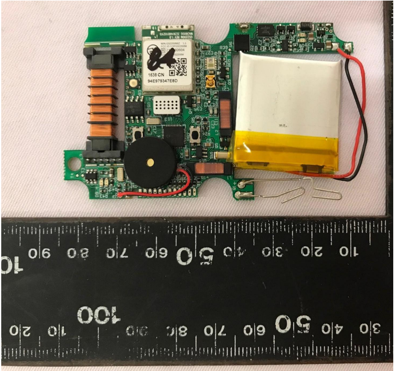
Main-Board PCB Component Side
