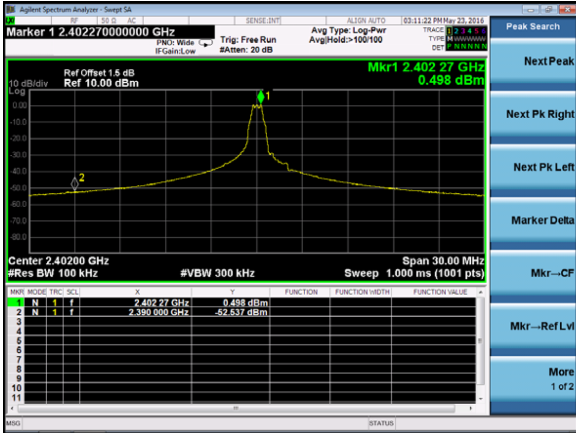
2402MHz Mark delta=53.035dB
