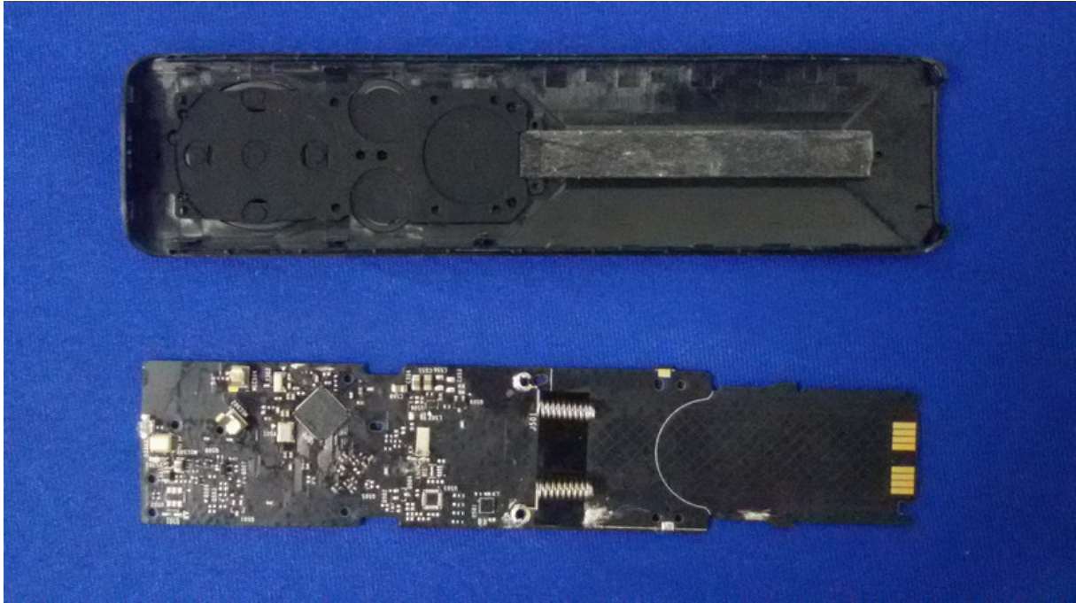
Figure 9 Inside of the EUT
