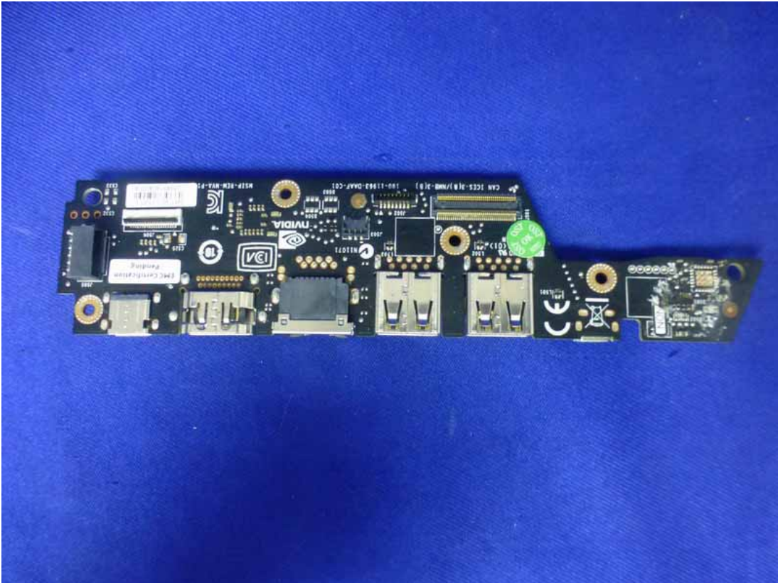
Figure 12 Front Side of the EUT
