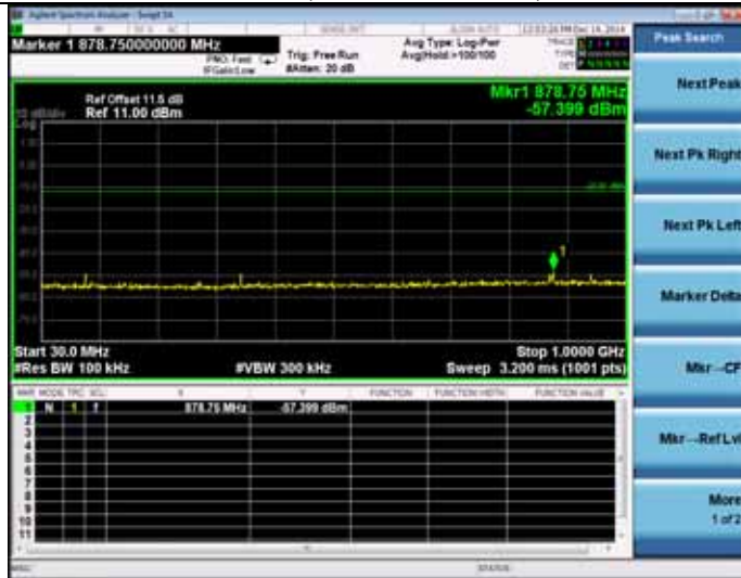
Test CH4: 2437MHz(30MHz – 1GHz)
