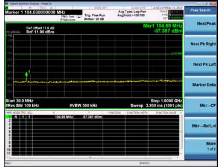
Test Mode: IEEE 802.11n HT40 TX Test CH1: 2422MHz(30MHz – 1GHz)
