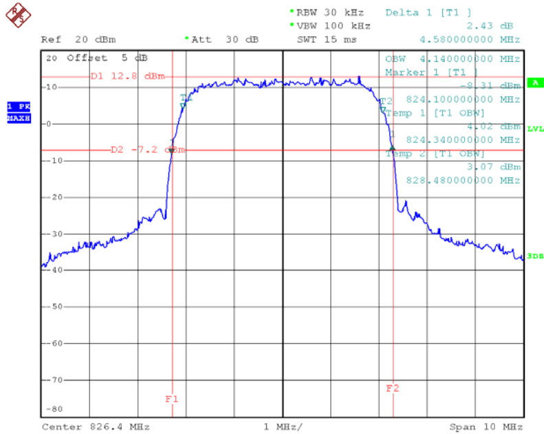
99% Occupied Bandwidth channel 4132
