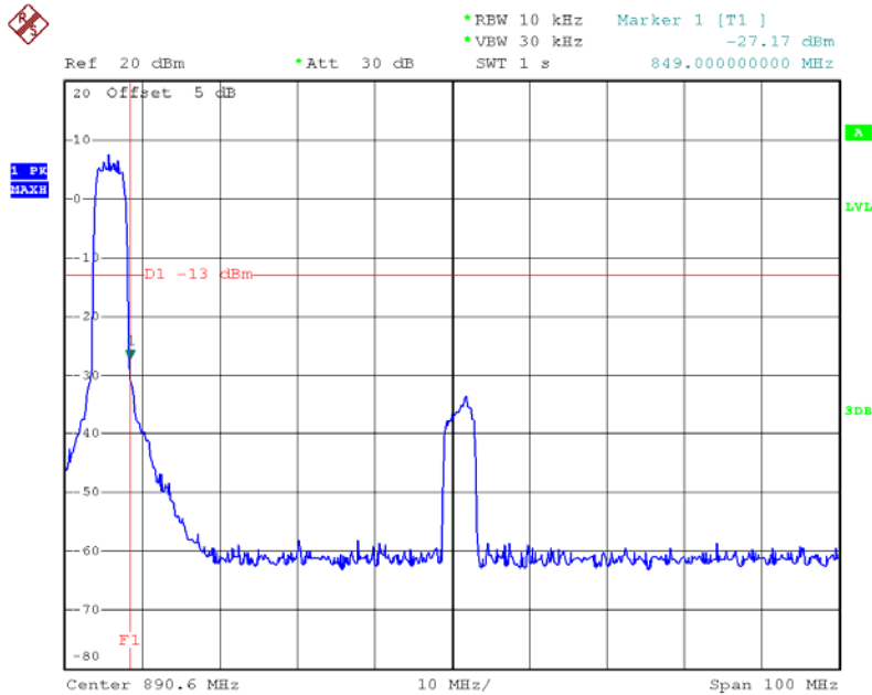
Band Edge on Configuration WCDMA- 12.2K RMC / Channel 4233-CONDUCTED MODE
