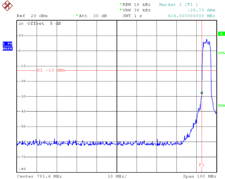
Band Edge on Configuration WCDMA- 12.2K RMC / Channel 4132-CONDUCTED MODE
