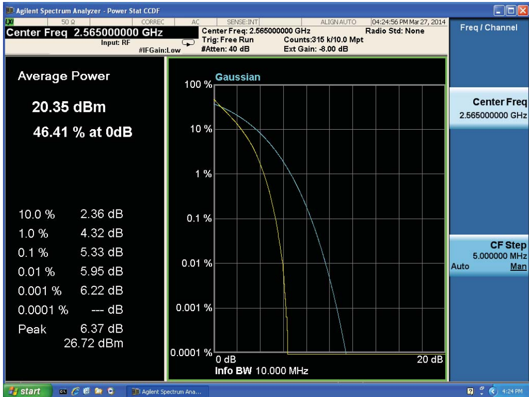
LTE Band 7 QPSK Bandwidth = 10MHz CH21400
