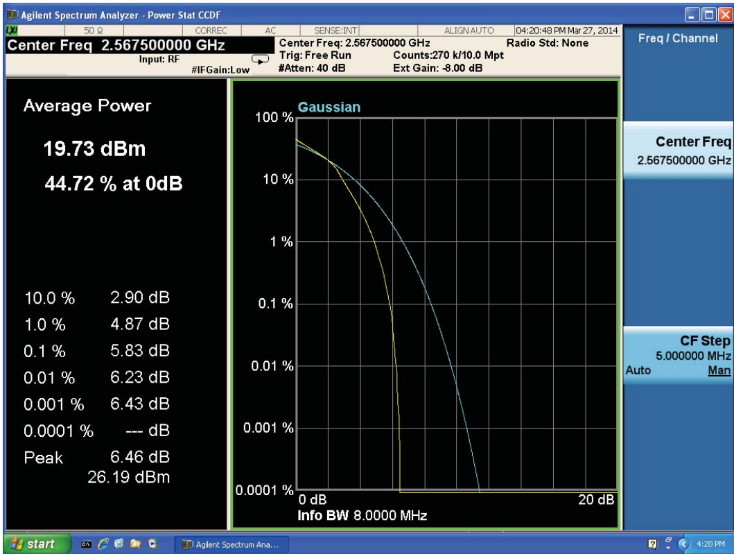
LTE Band 7 16QAM Bandwidth = 5MHz CH21425
