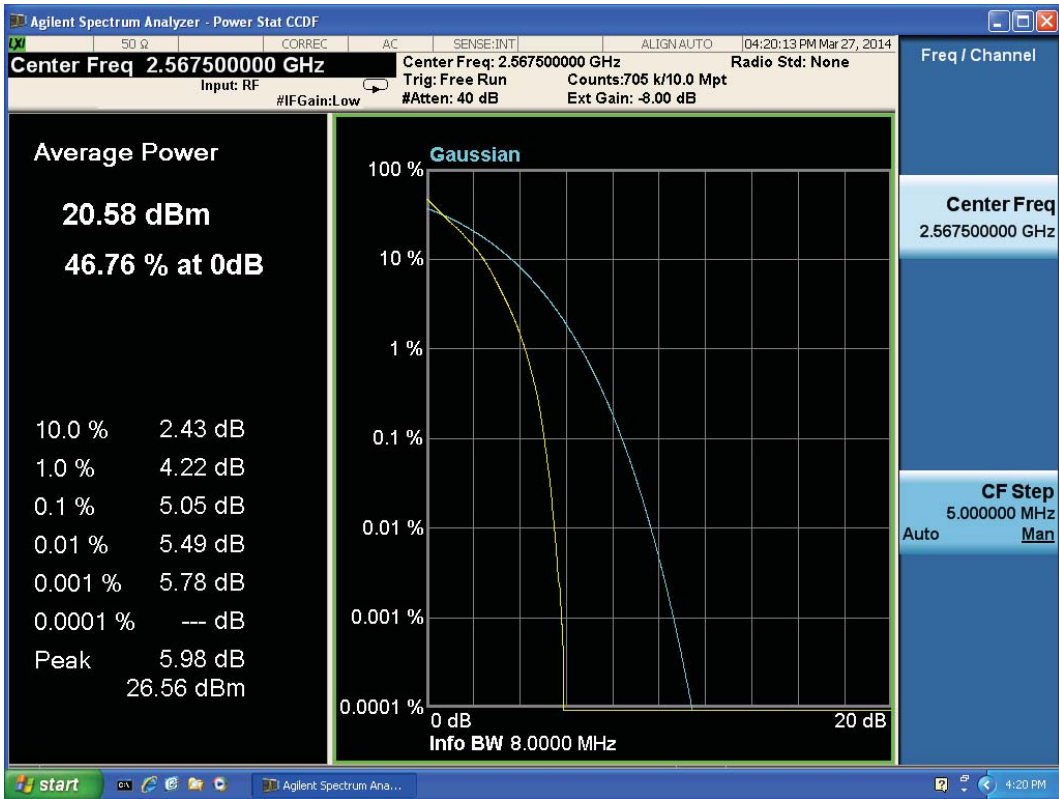
LTE Band 7 QPSK Bandwidth = 5MHz CH21425
