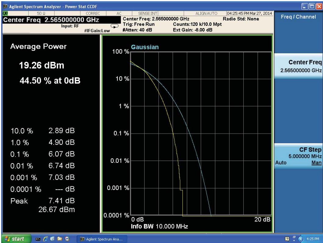
LTE Band 7 16QAM Bandwidth = 10MHz CH21400
