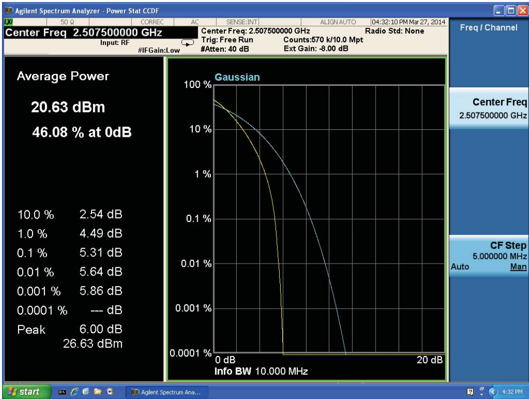
LTE Band 7 QPSK Bandwidth = 15MHz CH20825
