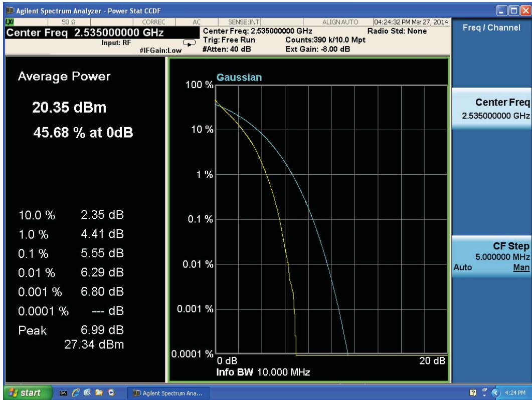
LTE Band 7 QPSK Bandwidth = 10MHz CH21100
