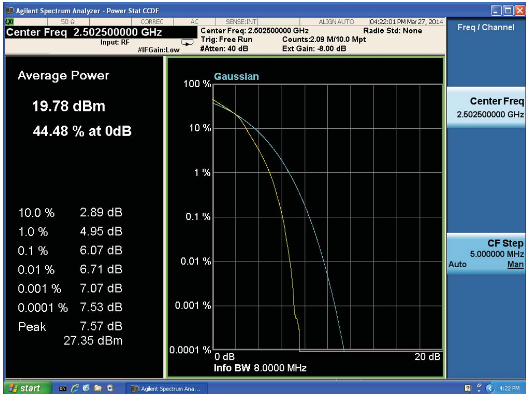
LTE Band 7 16QAM Bandwidth = 5MHz CH20775
