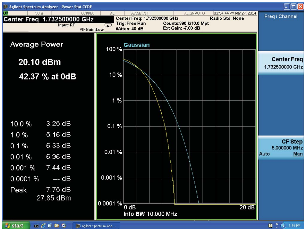
LTE Band 4 16QAM Bandwidth = 20MHz CH20175
