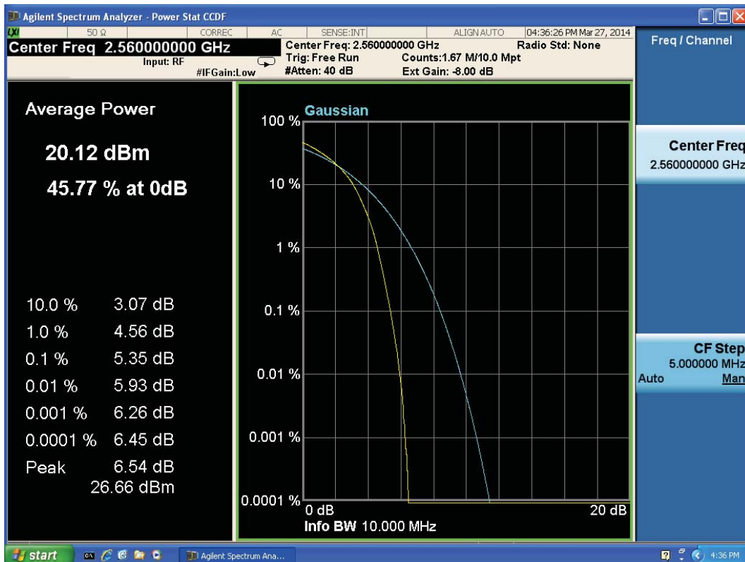
LTE Band 7 QPSK Bandwidth = 20MHz CH21350
