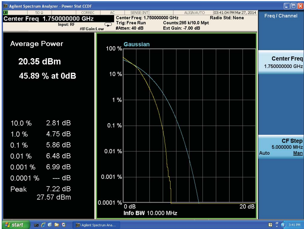
LTE Band 4 16QAM Bandwidth = 10MHz CH20350
