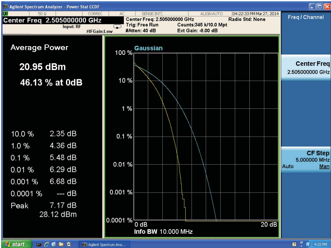
LTE Band 7 QPSK Bandwidth =10MHz CH20800
