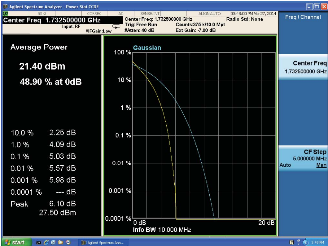
LTE Band 4 QPSK Bandwidth = 10MHz CH20175
