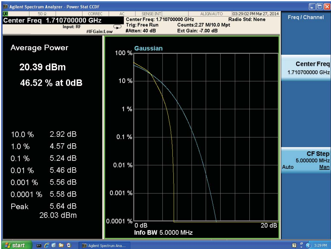
LTE Band 4 16QAM Bandwidth = 1.4MHz CH19957
