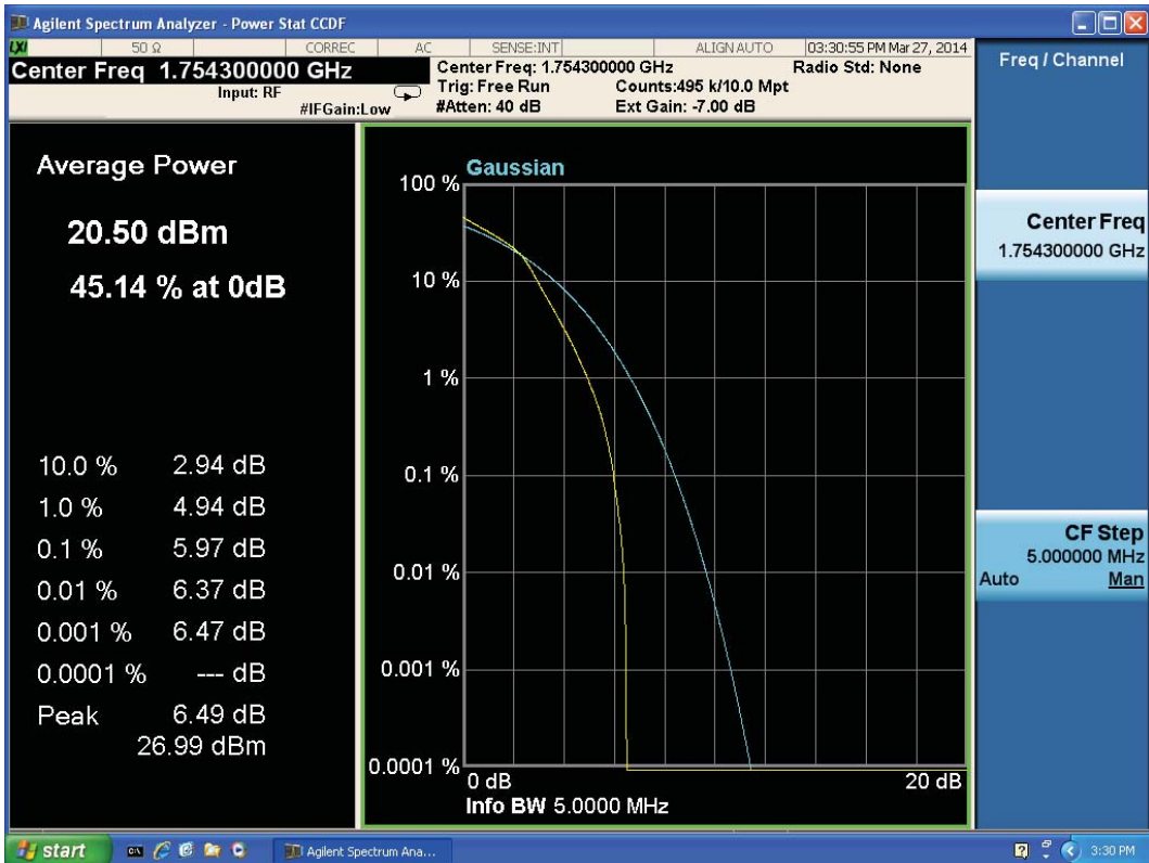
LTE Band 4 16QAM Bandwidth = 1.4MHz CH20393
