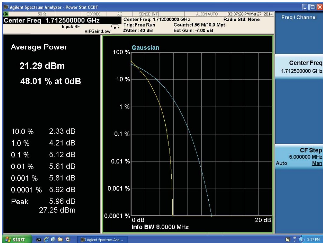
LTE Band 4 QPSK Bandwidth = 5MHz CH19975
