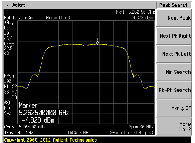
802.11n-HT20 mode, 5260 MHz, Chain 1
