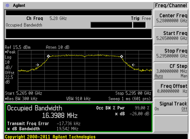
802.11a mode, 5280 MHz, Chain 1
