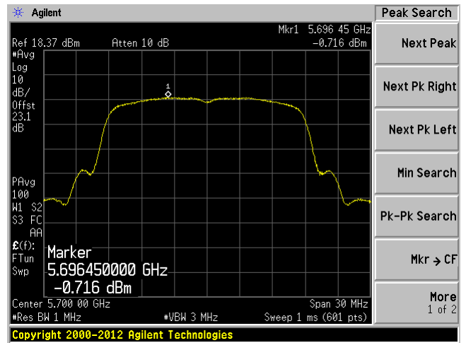
802.11n-HT20 mode, 5700 MHz, Chain 1
