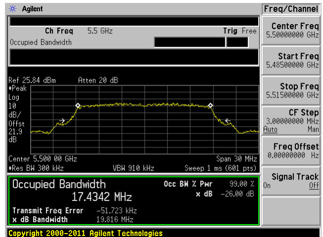
802.11n-HT20 mode, 5500 MHz, Chain 1
