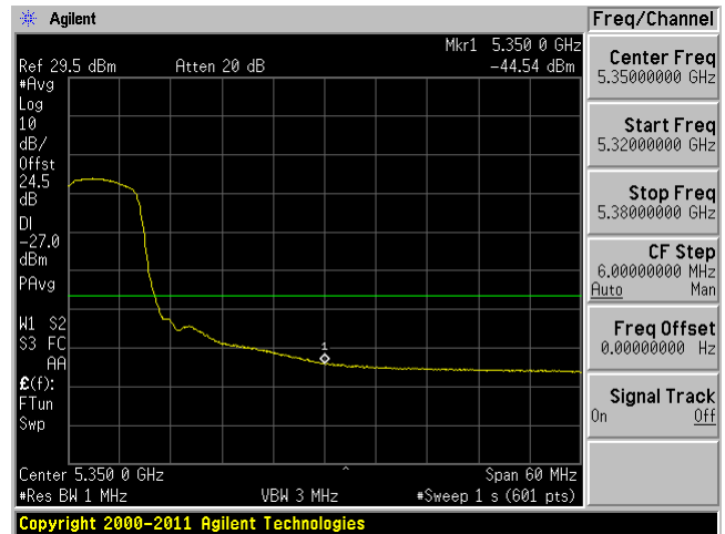
802.11a mode, 5320 MHz, Chain 1
