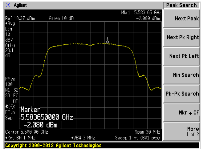
802.11n-HT20 mode, 5580 MHz, Chain 1
