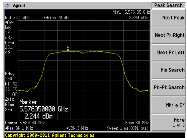
802.11a mode, 5580 MHz, Chain 1
