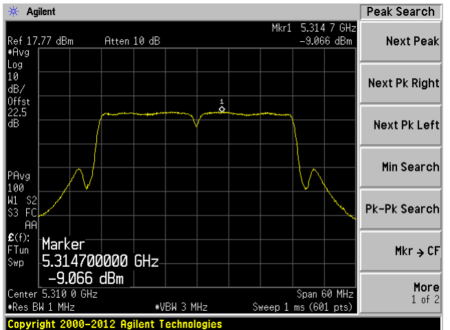
802.11n-HT40 mode, 5310 MHz, Chain 1
