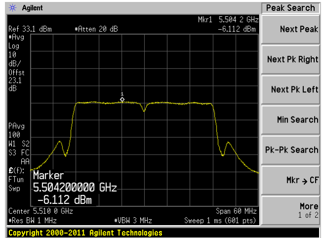
802.11n-HT40 mode, 5510 MHz, Chain 1
