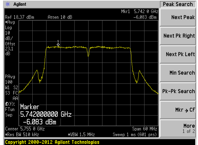
Low channel: 5755 MHz Chain 1
