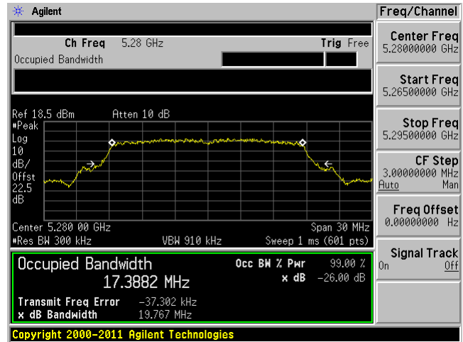
802.11n-HT20 mode, 5280 MHz, Chain 1
