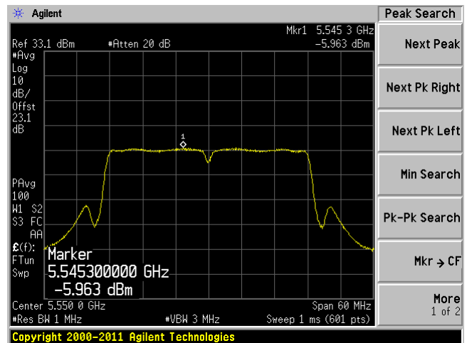
802.11n-HT40 mode, 5550 MHz, Chain 1
