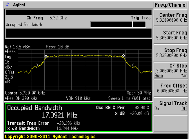
802.11n-HT20 mode, 5320 MHz, Chain 1
