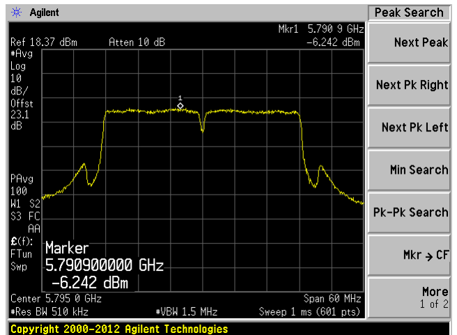
High channel: 5795 MHz Chain 1
