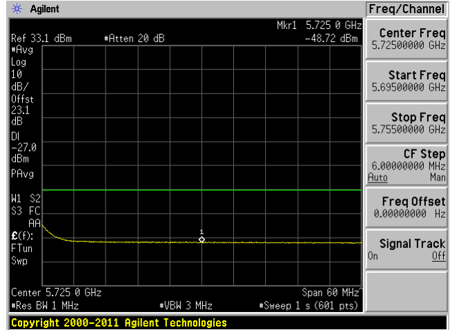
802.11n-HT40 mode, 5670 MHz, Chain 1
