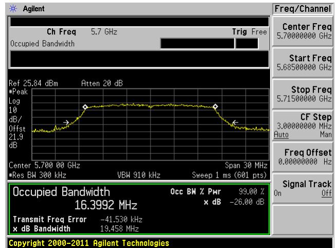
802.11a mode, 5700 MHz, Chain 1
