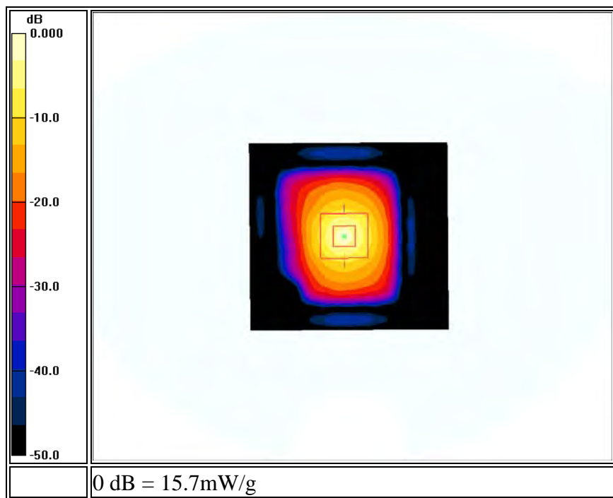
5500 MHz System Validation with Body Tissue
