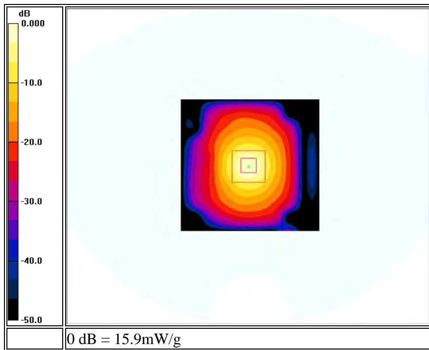
5200 MHz System Validation with Body Tissue
