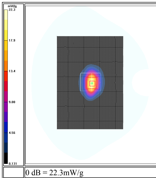
1900 MHz System Validation with Body Tissue
