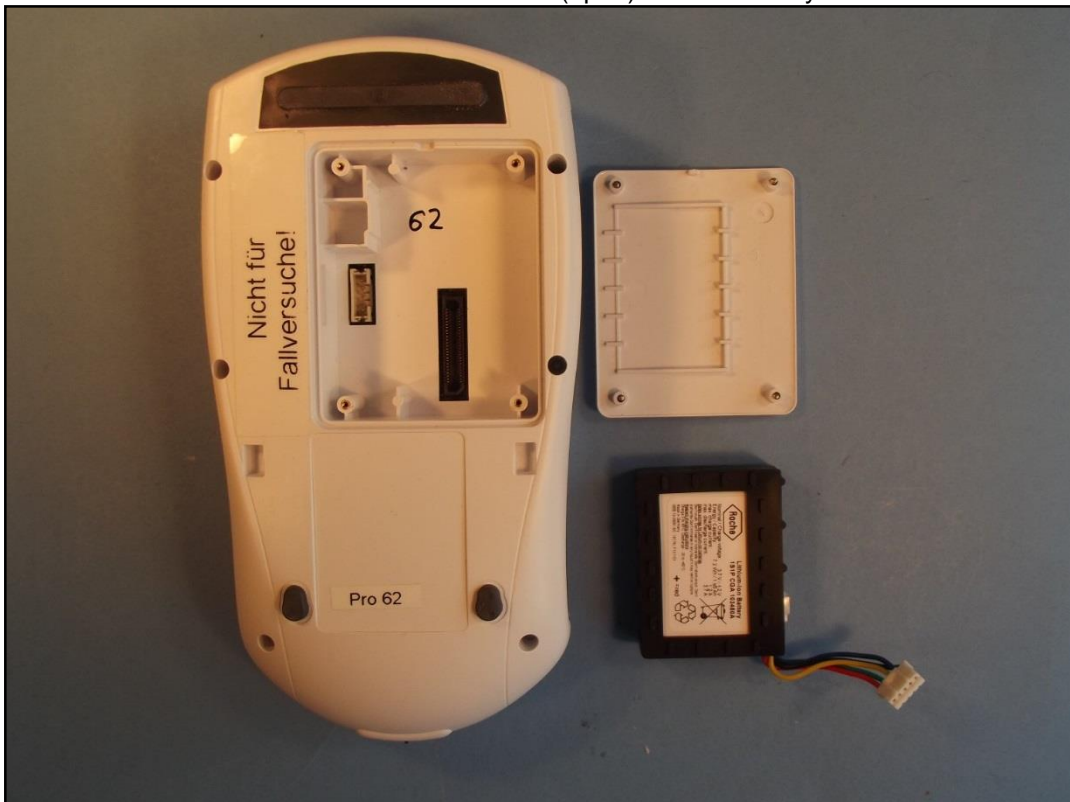
Photo 8: DUT - rear view (open) without battery
