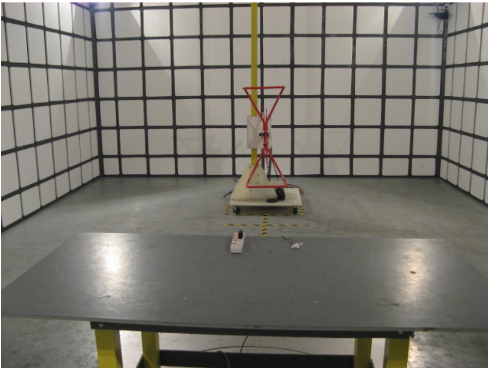
RADIATED EMISSION TEST SETUP – CHARGING
