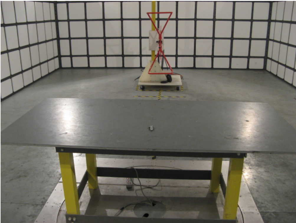
RADIATED EMISSION TEST SETUP - TRANSMITTING
