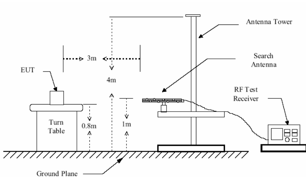
Figure 1 : Frequencies measured below 1 GHz configuration
