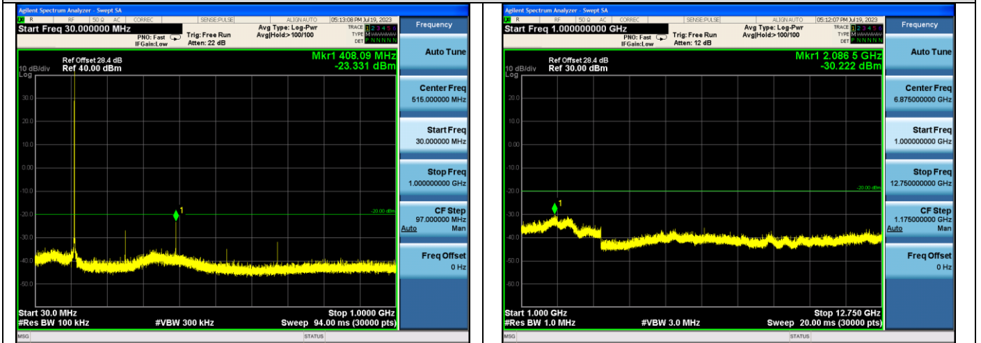
12.5kHz, Analog modulation, Assigned Frequency: 155.025MHz,
