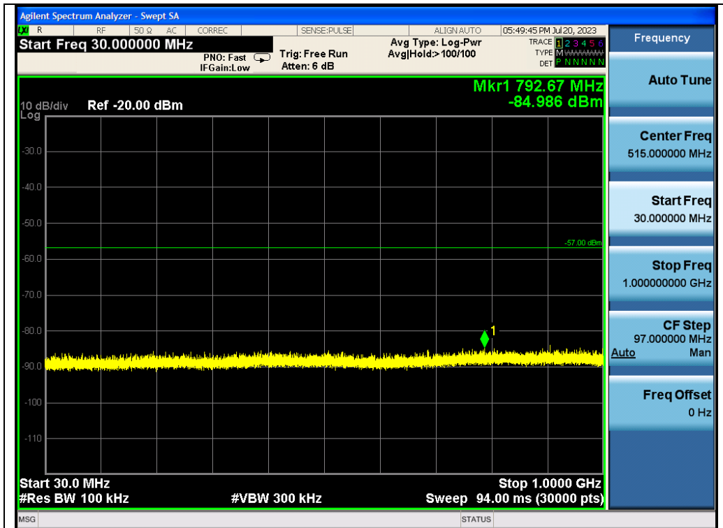
Test_Graph_RX_FrequencyRange_30MHz-1GHz
