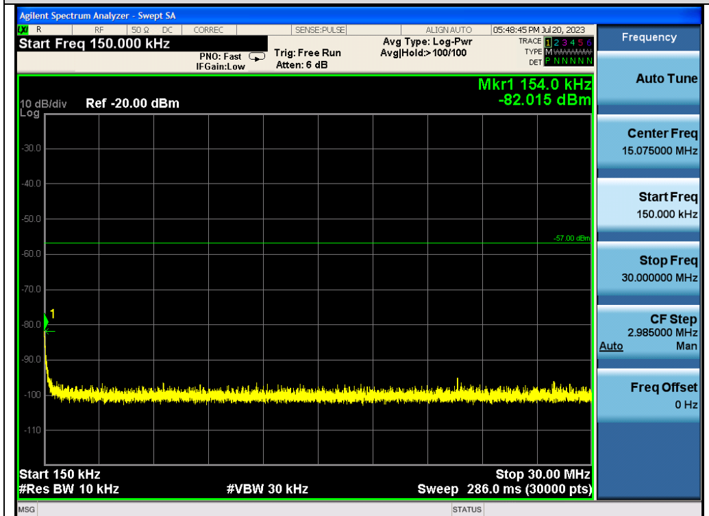
Test_Graph_RX_FrequencyRange_150kHz-30MHz
