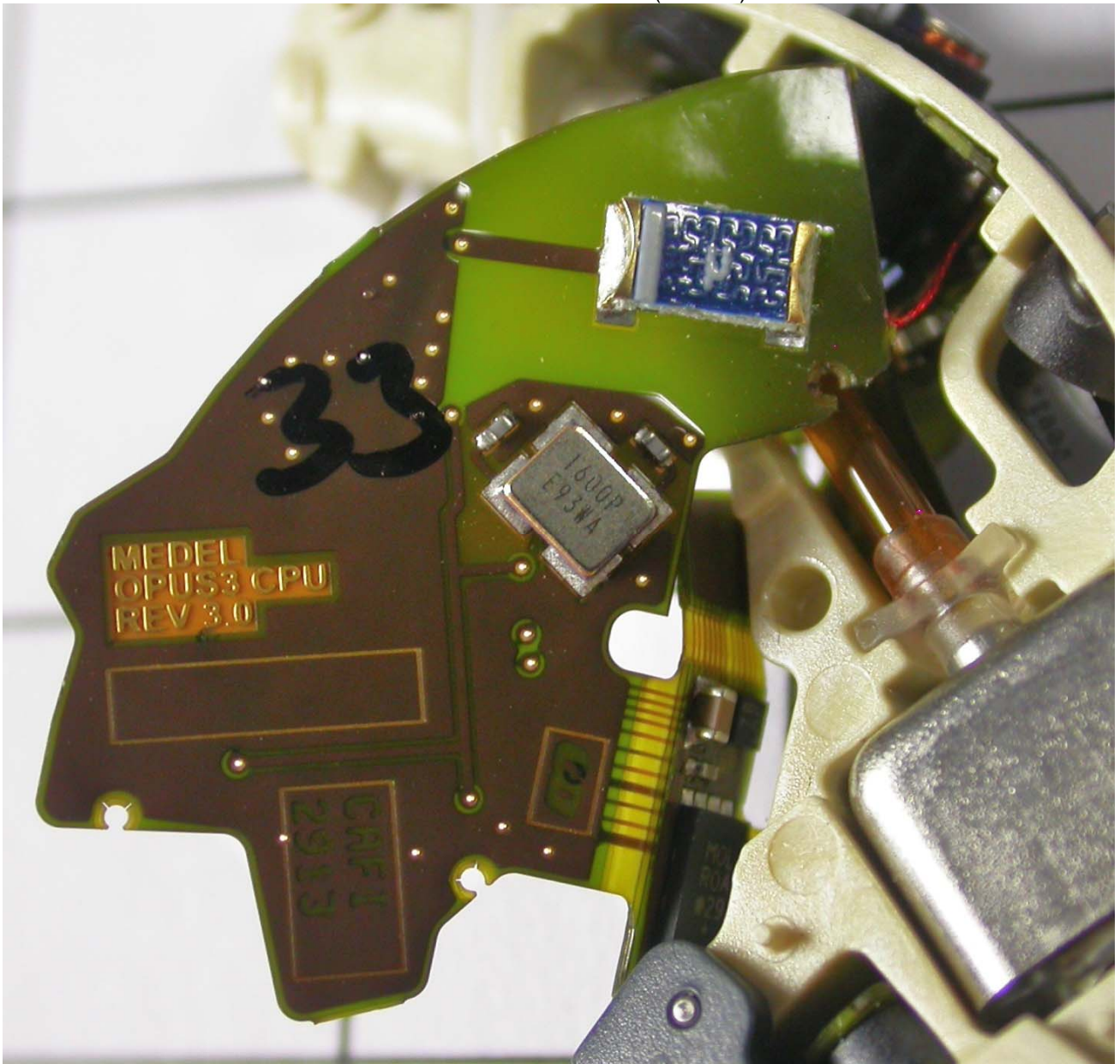
PCB bottom / antenna view (left side)
