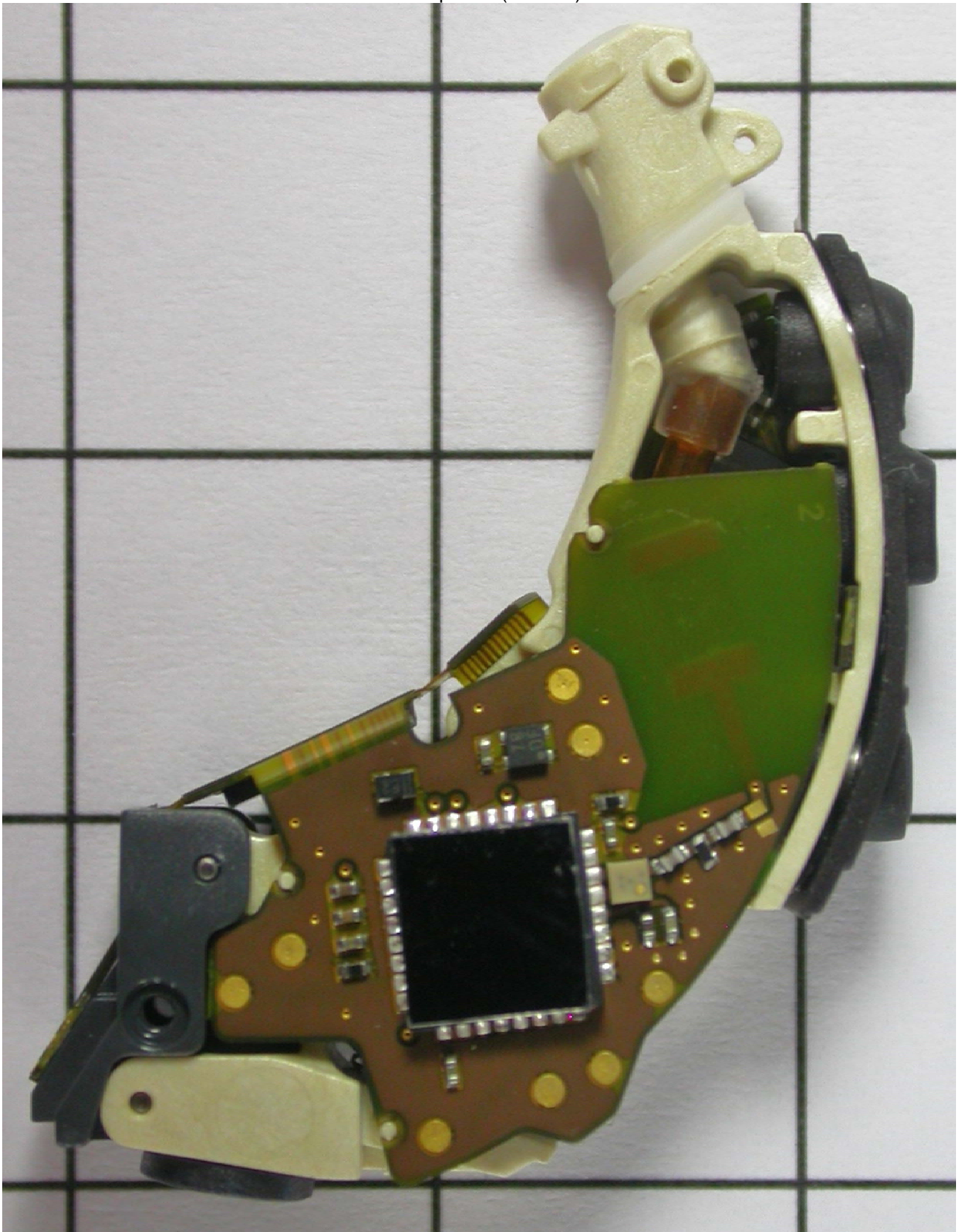
PCB top view (left side)
