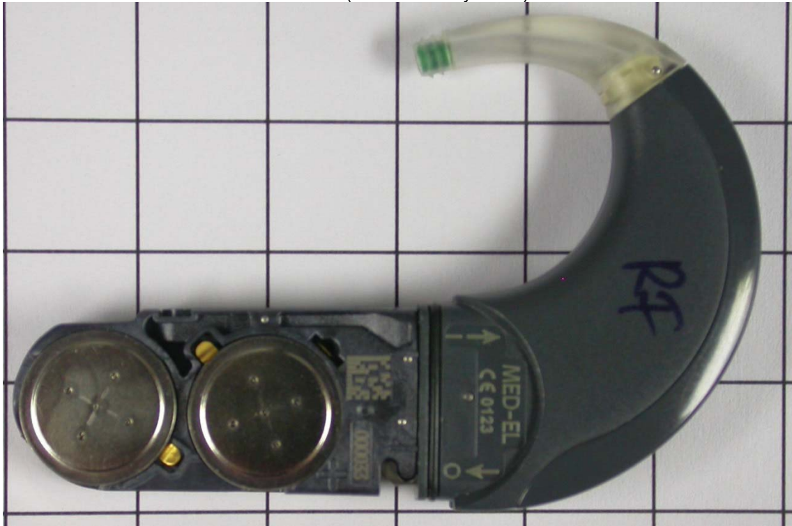
Right view (without battery cover)
