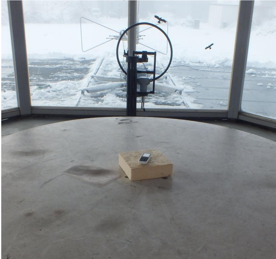
Test setup 9 kHz – 30 MHz:
