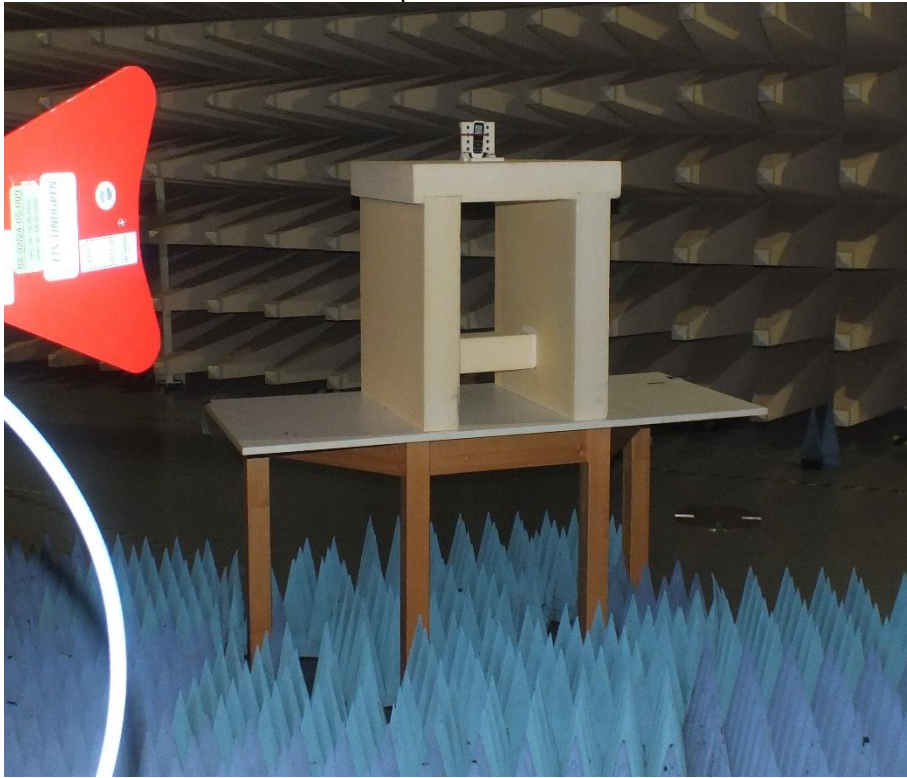
Test setup 1 GHz – 18 GHz:
