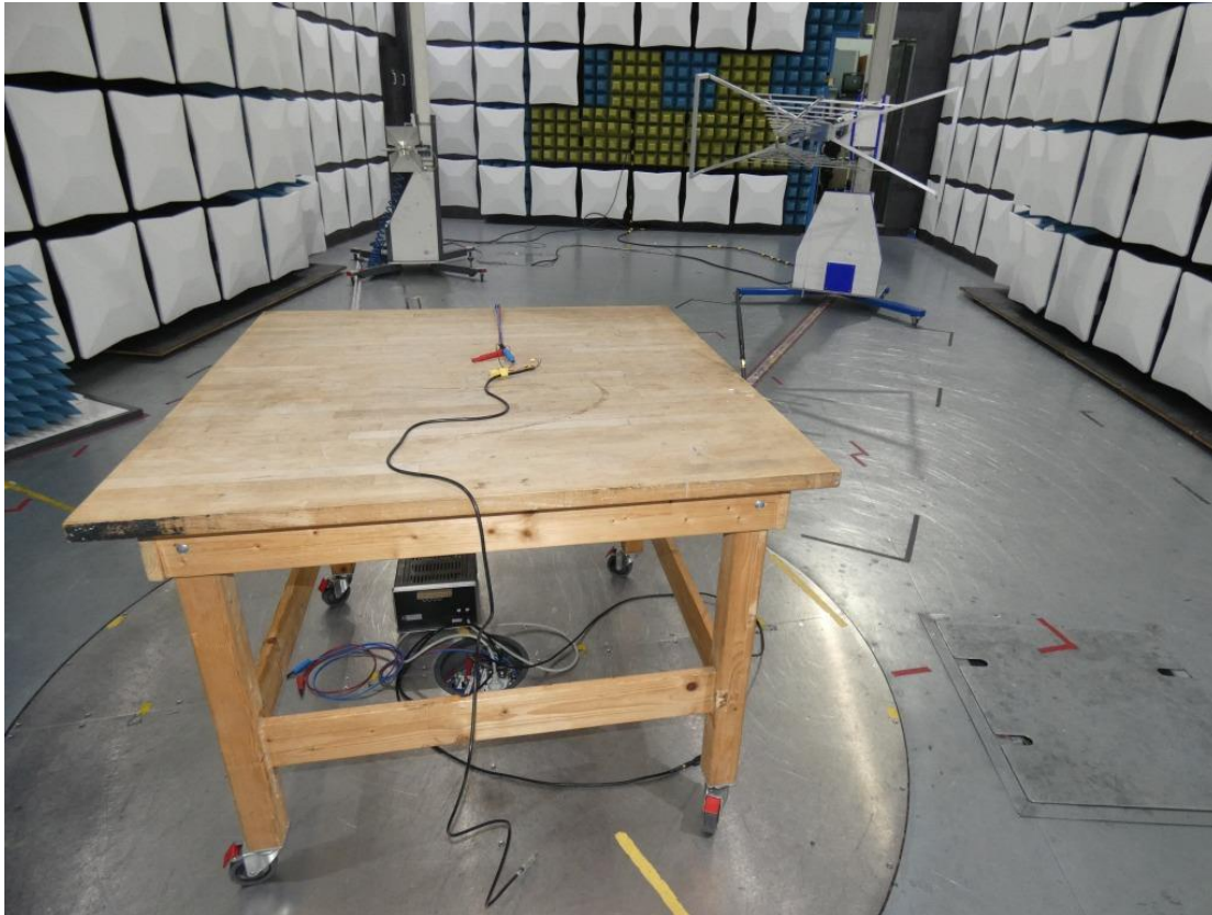
Photo 3: Test setup for radiated measurements (stand alone setup, 30 MHz - 1 GHz; FCC 15c247)
