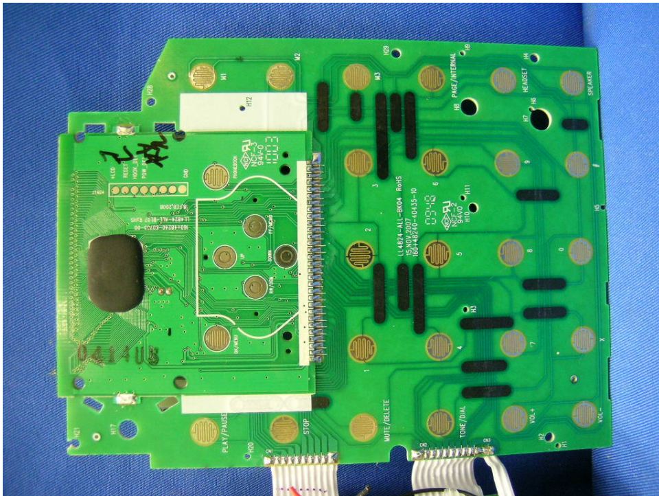
Base Unit Keypad PCB front side (View 2)
