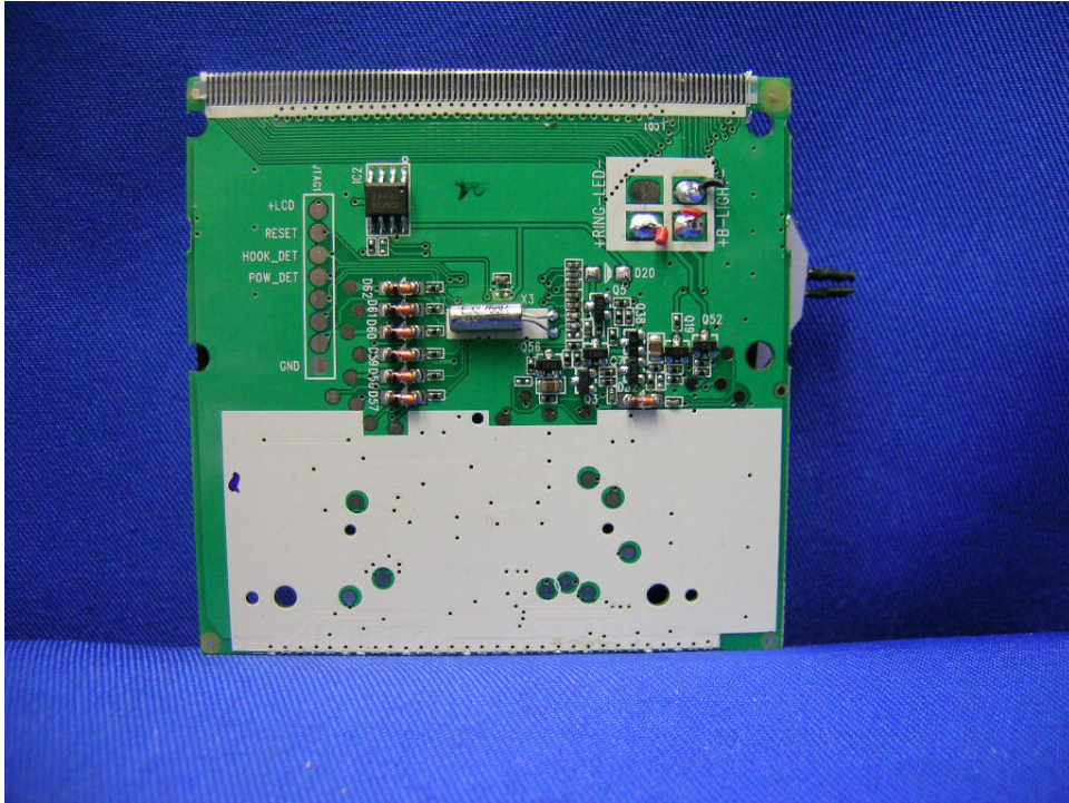
Base Unit LCD Board front side (View 2)
