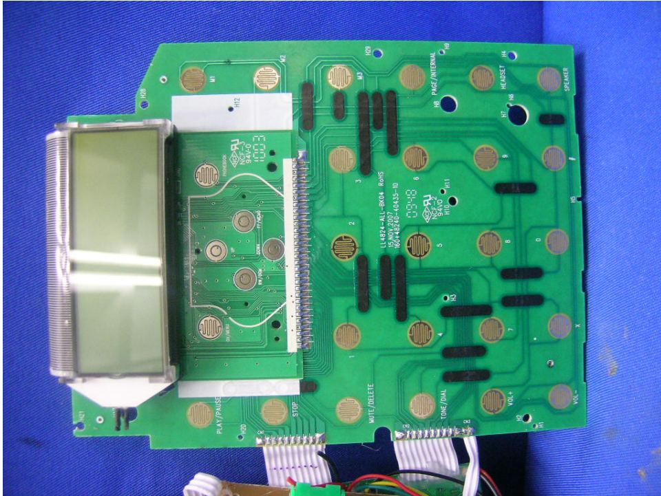
Base Unit Keypad PCB front side (View 1)
