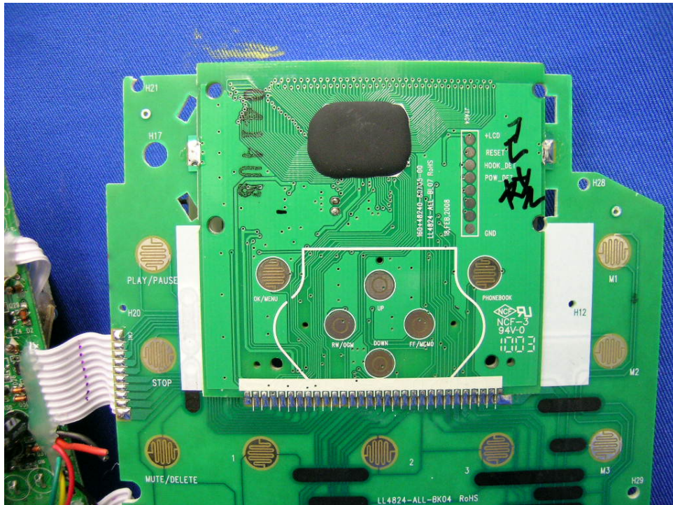
Base Unit LCD Board front side (View 1)
