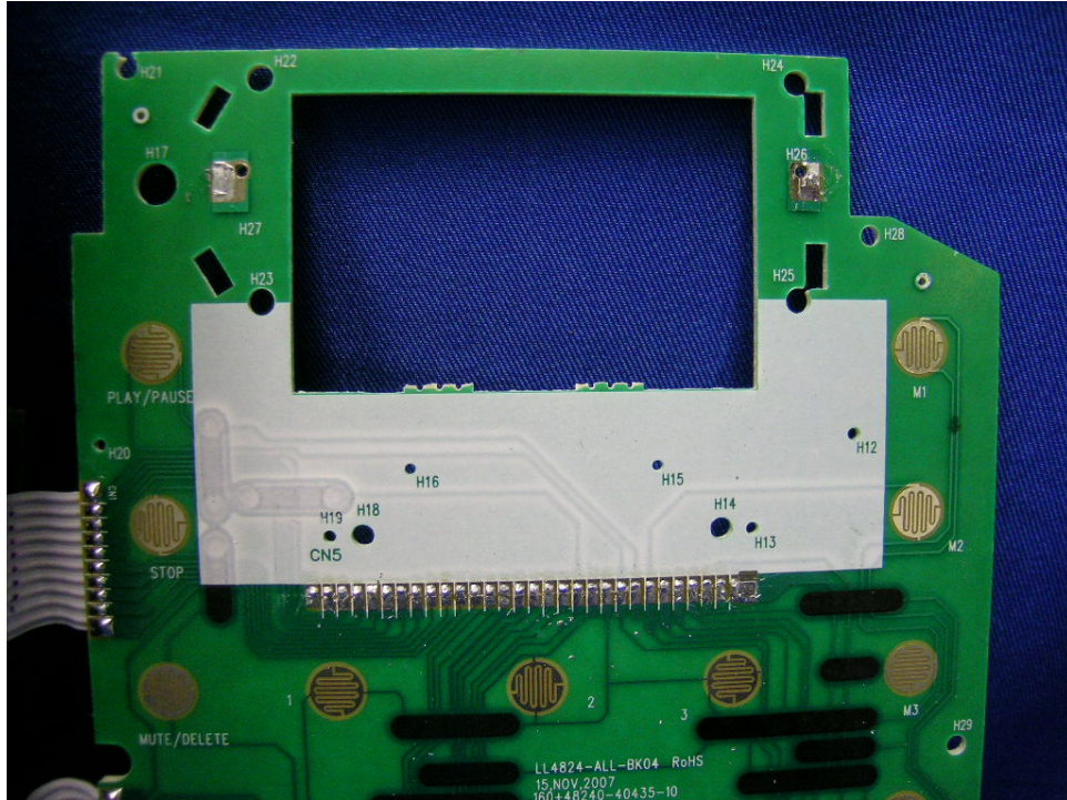
Base Unit Keypad PCB front side (View 3)
