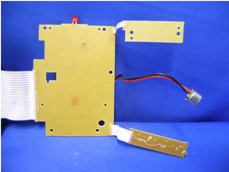
Base Unit Keypad PCB rear side
