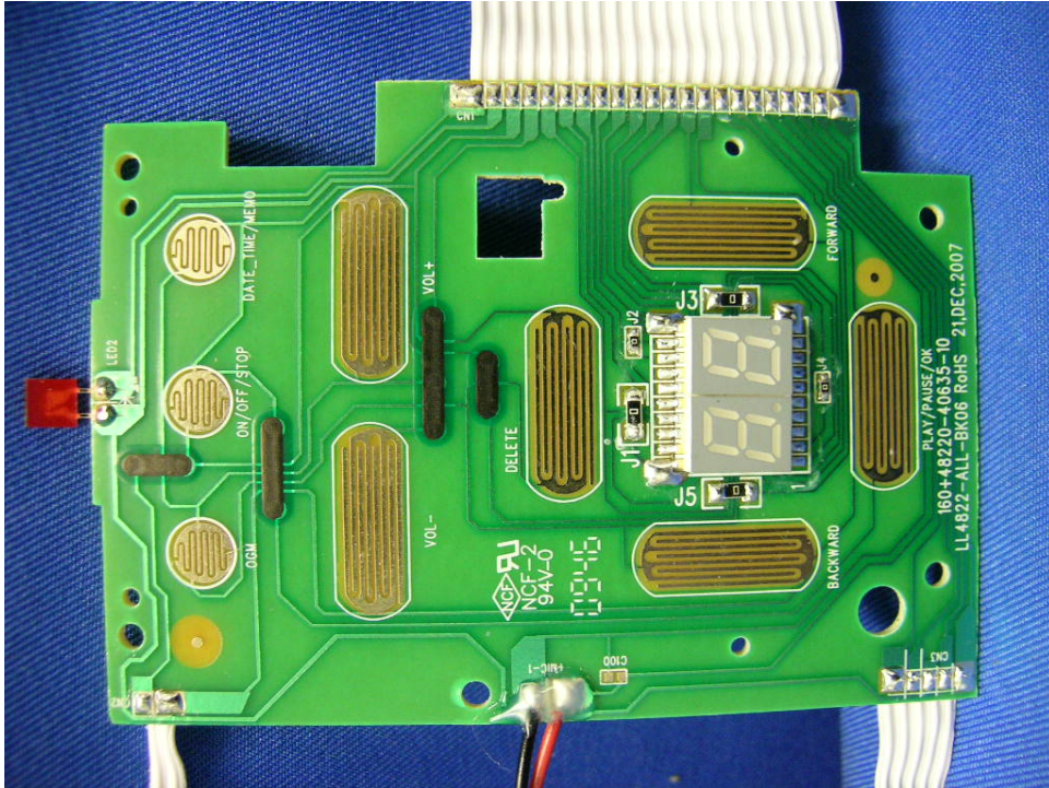
Base Unit Keypad PCB front side
