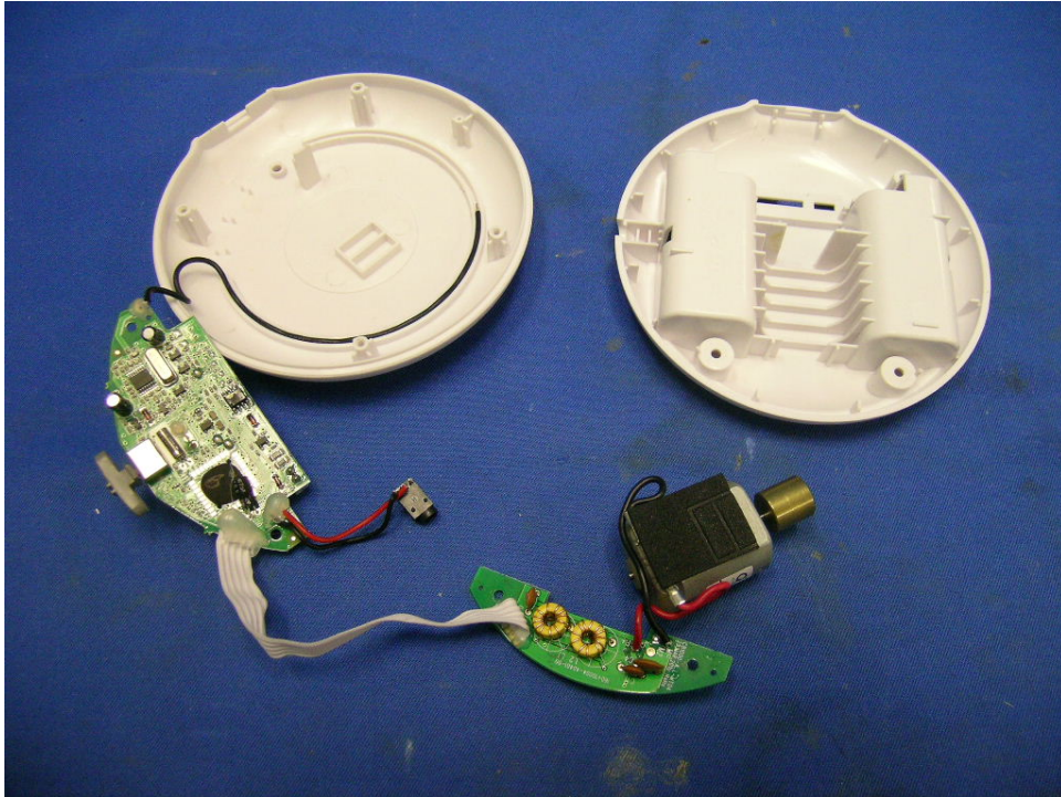
Bed Shaker assembly (View 2)
