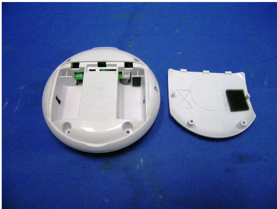
Bed Shaker Battery compartment
