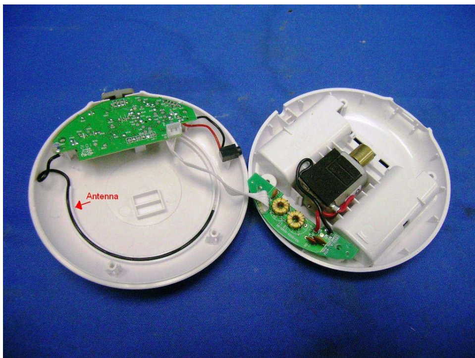
Bed Shaker assembly (View 1)
