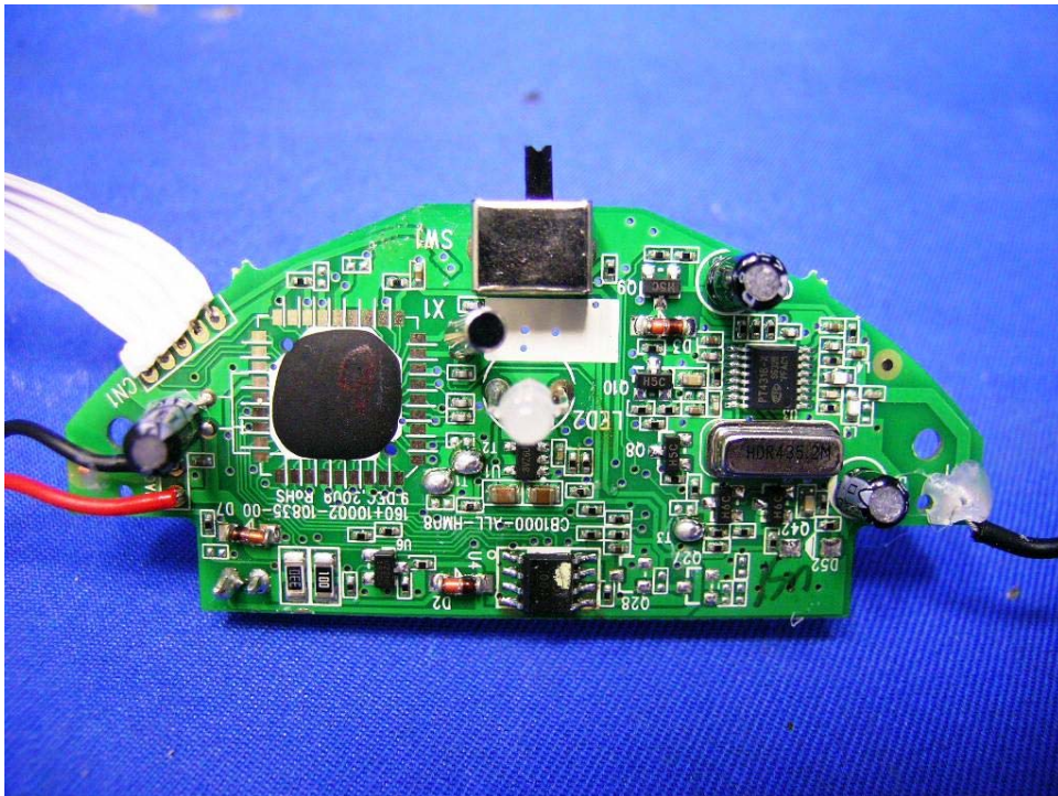
Bed Shaker Main PCB comp side
