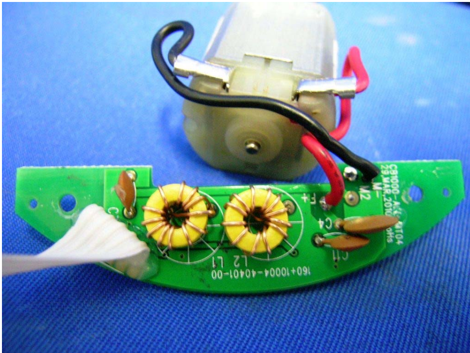
Bed Shaker Vibrator PCB comp side
