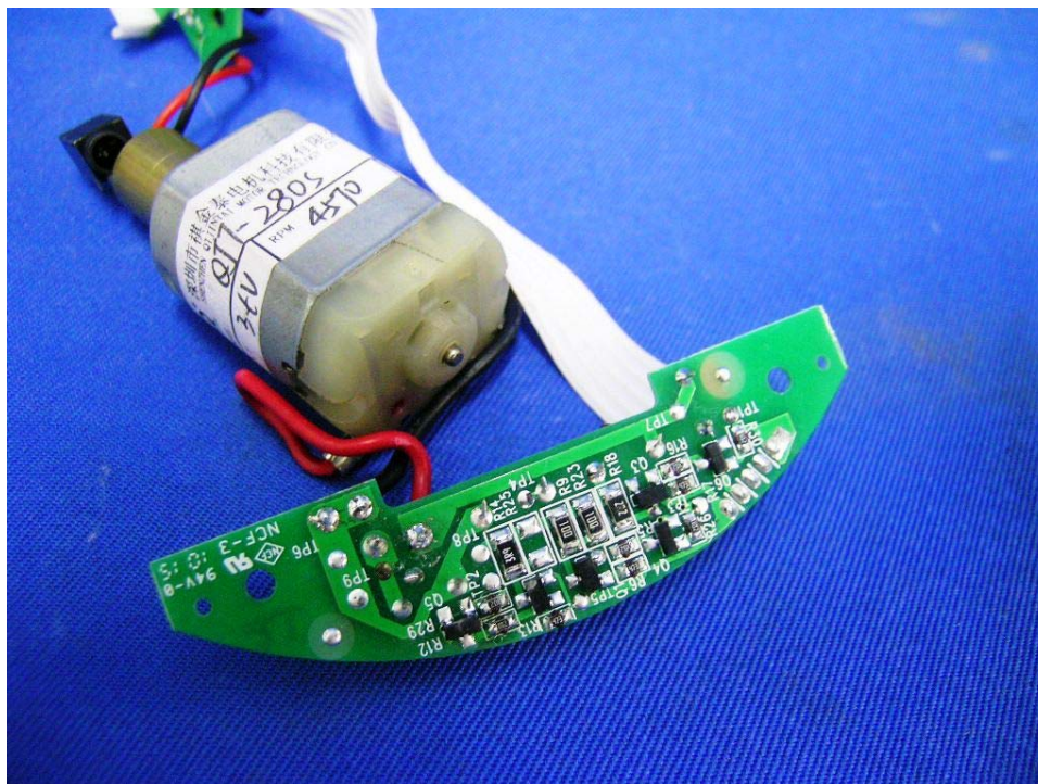
Bed Shaker Vibrator PCB solder side
