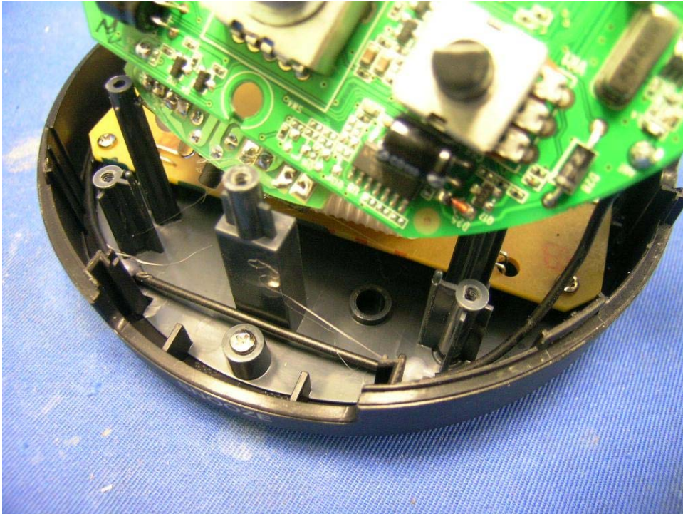
Alarm Clock Antenna location
