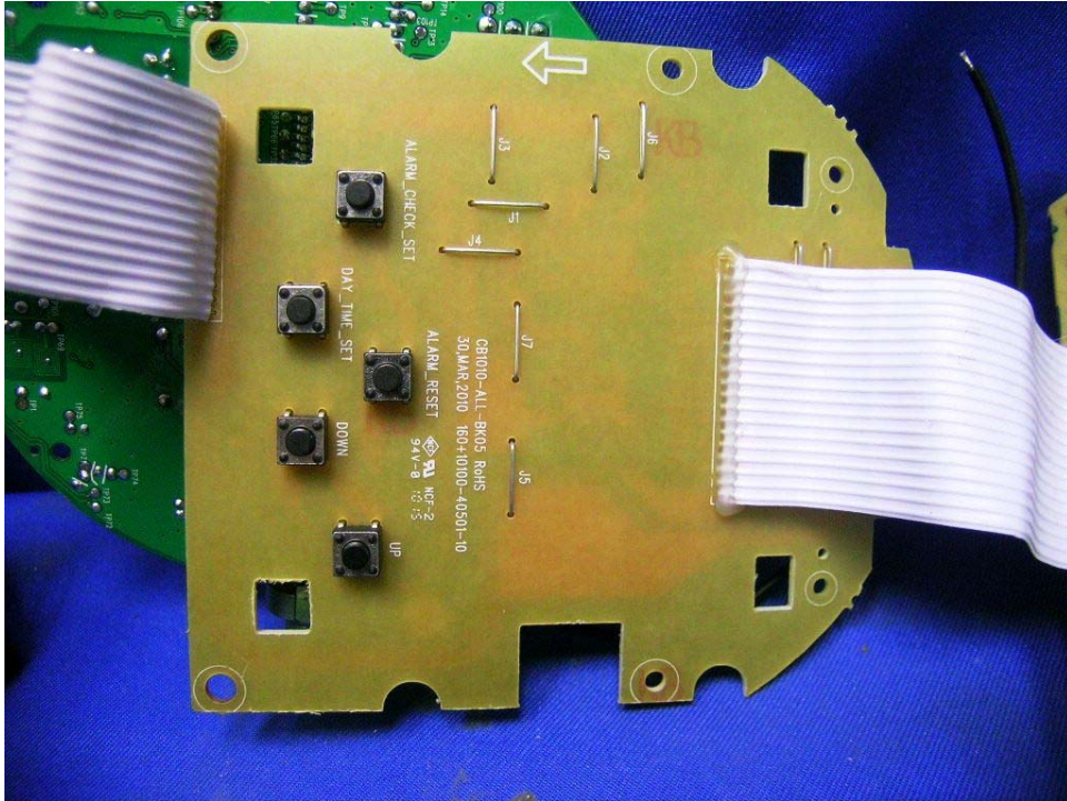
Alarm Clock PCB comp side (View 1)
