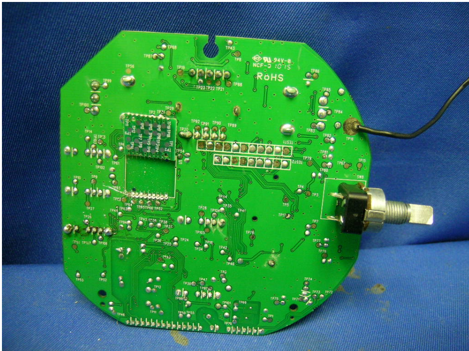
Alarm Clock Main PCB solder side (View 2)
