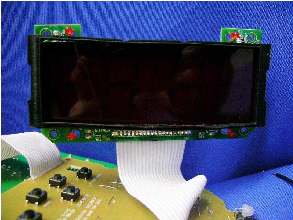
Alarm Clock Display PCB comp side (View 1)
