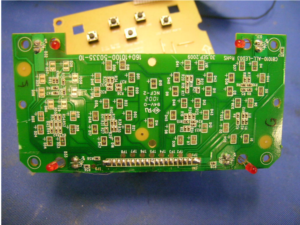
Alarm Clock Display PCB comp side (View 2)
