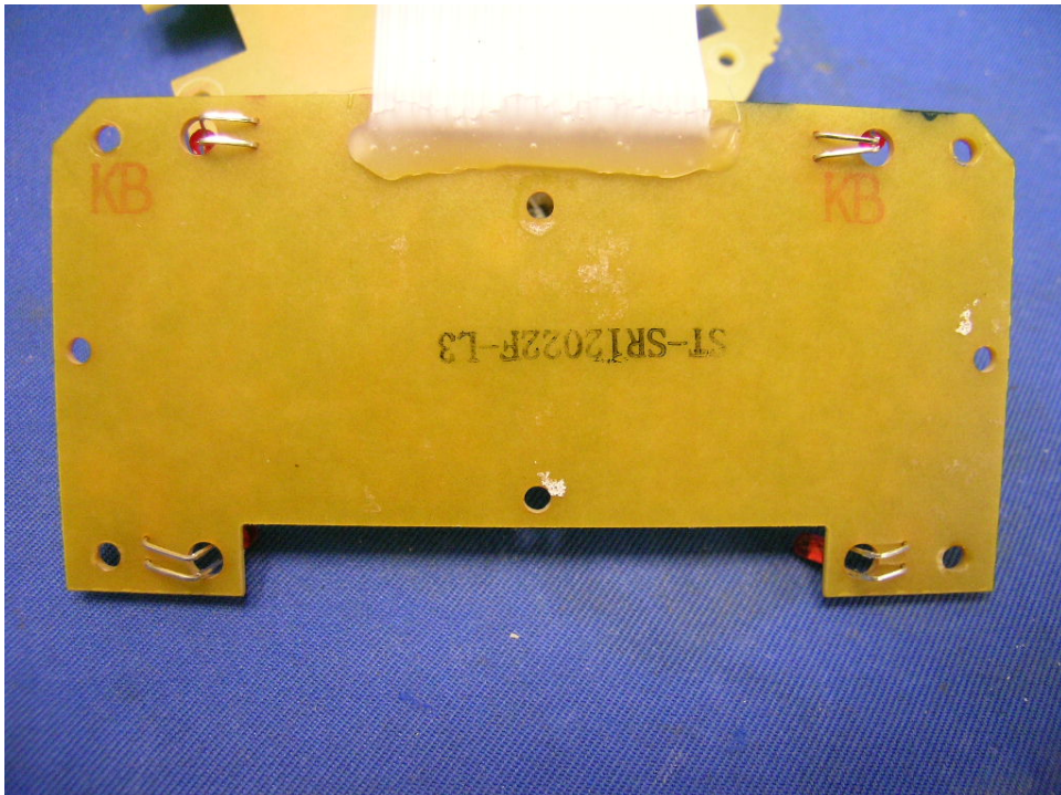
Alarm Clock Display PCB solder side
