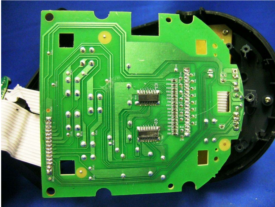
Alarm Clock PCB solder side
