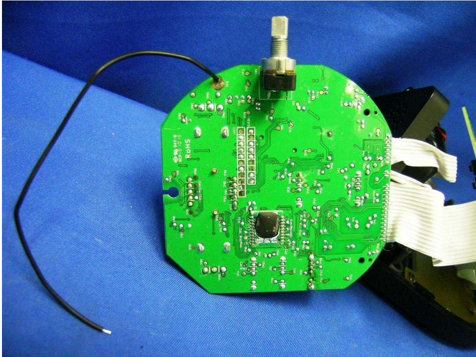
Alarm Clock Main PCB solder side (View 1)
