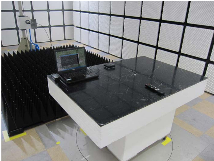
Radiated RF measurement (Above 1 GHz)
