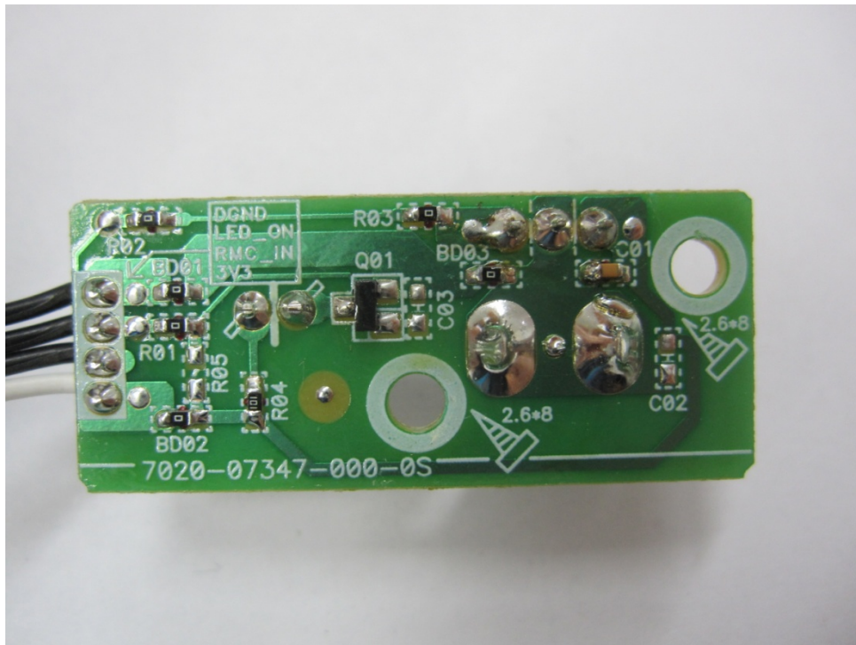
Connection Board Rear
