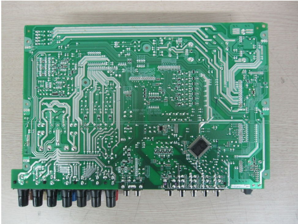
Power Board-1_Rear
