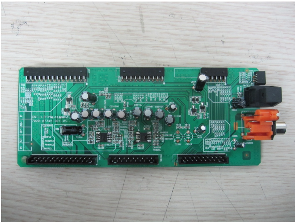
Connection Board Front-1
