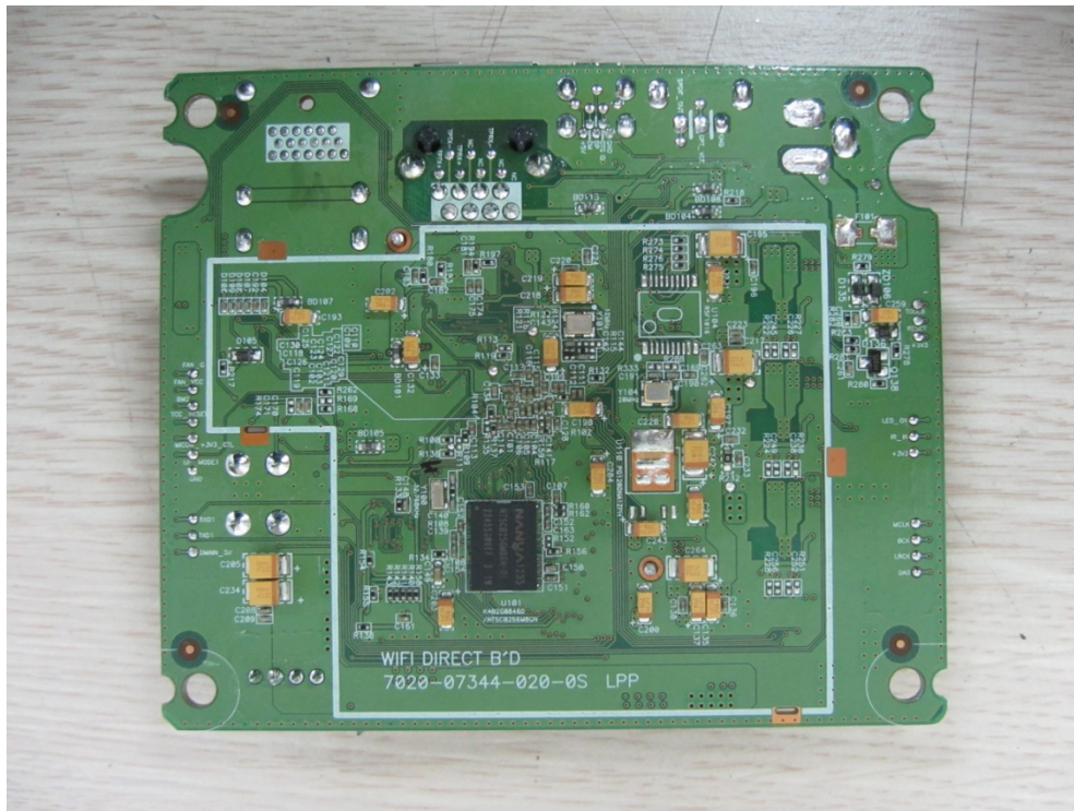
WIFI Board Rear
