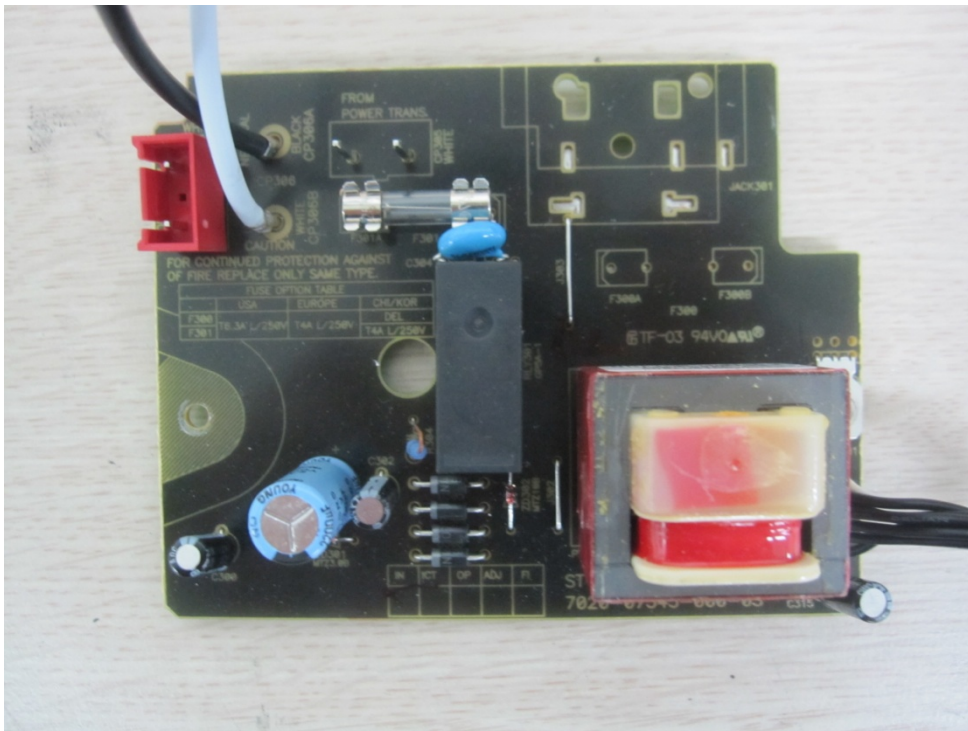
Power Board-3_Front
