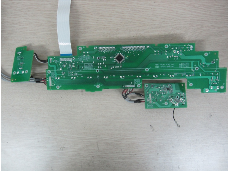
Display Board Rear
