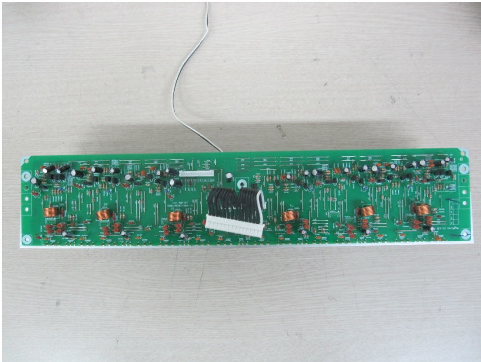
Power Board-2_Front
