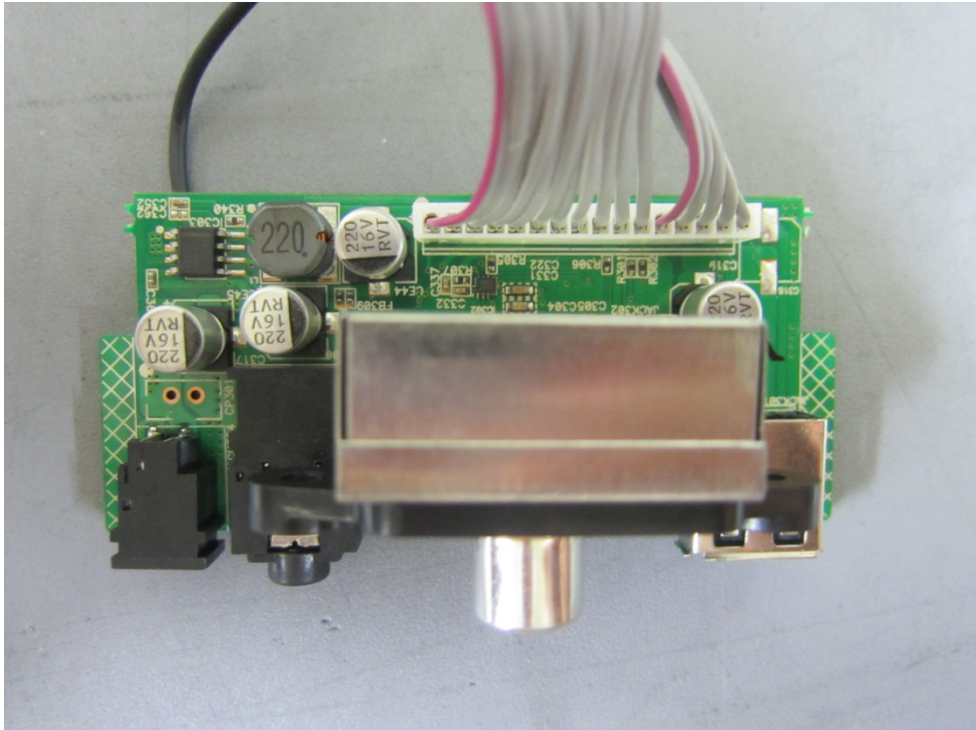
Sub Board_Front
