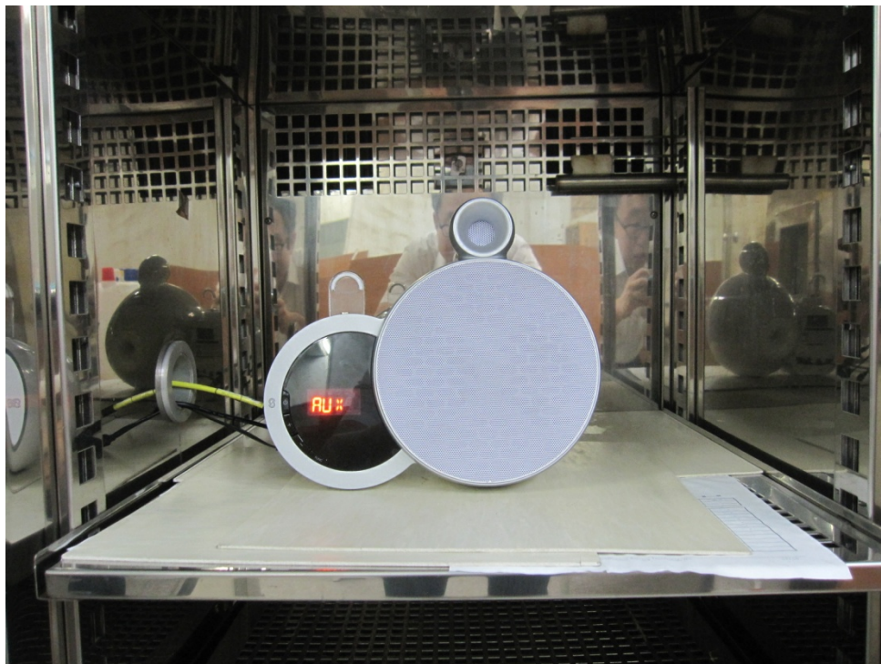
Conducted RF measurement within Temperature Chamber
