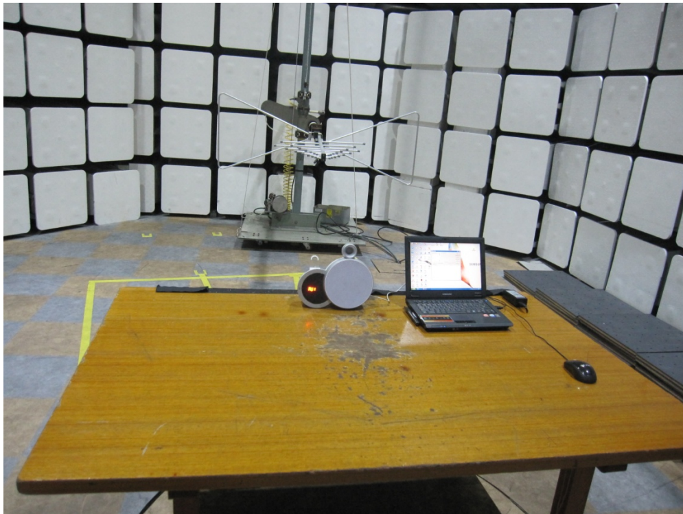
Radiated RF measurements (Below 1 GHz)
