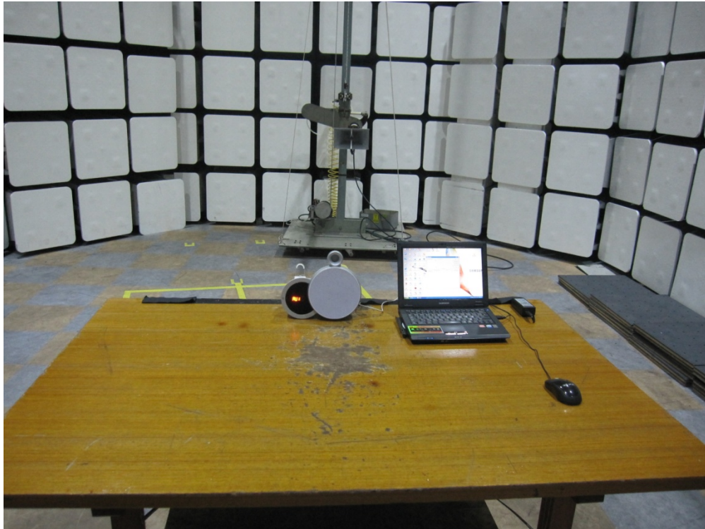
Radiated RF measurements (Above 1 GHz)
