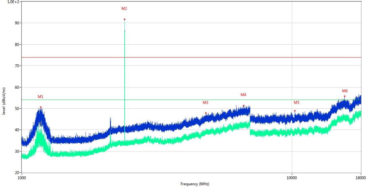
RE Test case_FCC Part 15C_FCC 15.247(2.4G)_1GHz-18GHz 1.0E+2
