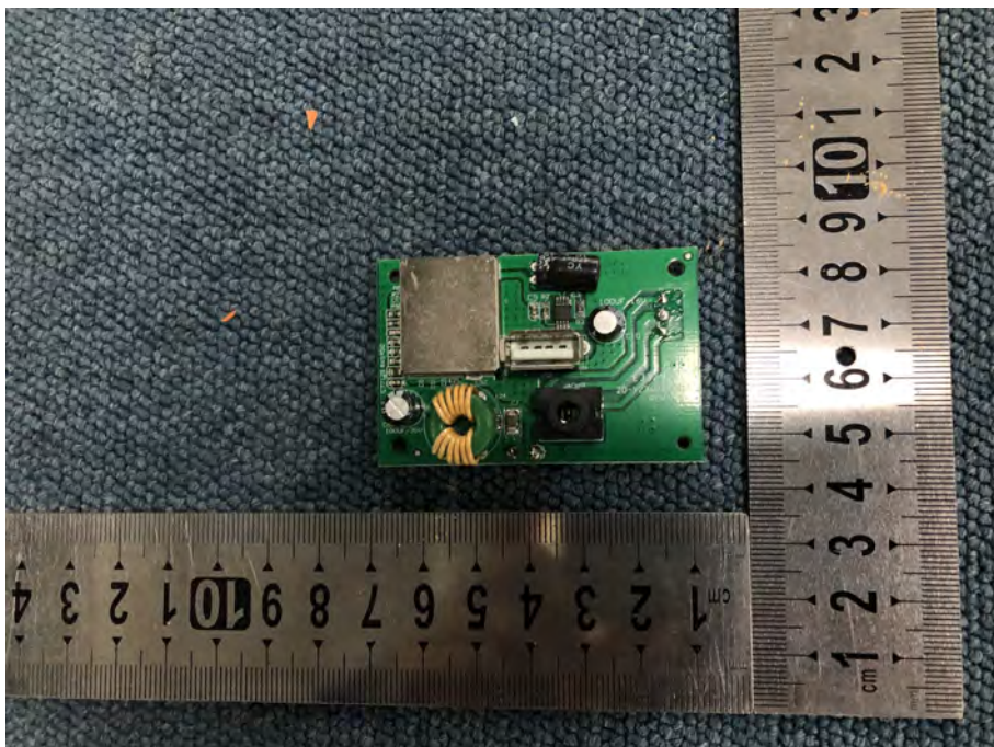
MAIN BOARD 2 FRONT VIEW(WITH SHIELDING)
