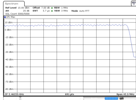
8-DPSK 2.4415 GHz ~ 2.4835 GHz
