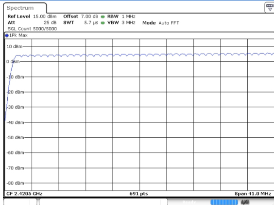
GFSK 2.4 GHz ~ 2.4415 GHz
