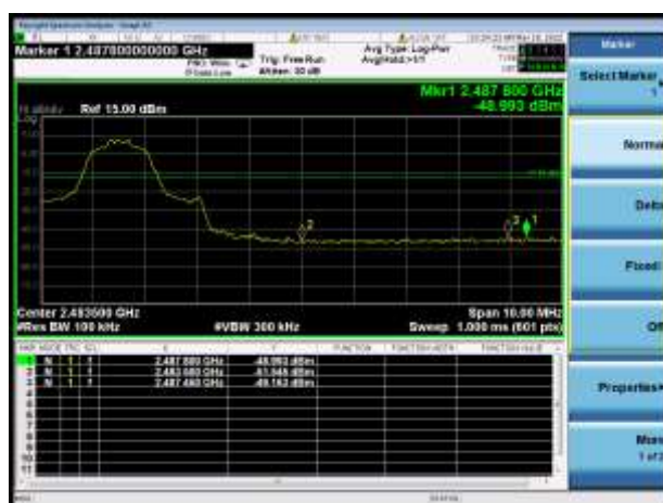
\pi/4 -DQPSK HIGH CHANNEL, BAND EDGE
