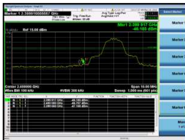
\pi/4 -DQPSK LOW CHANNEL, BAND EDGE
