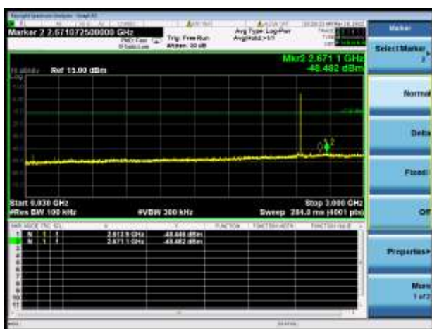
\pi/4 -DQPSK MIDDLE CHANNEL, SPURIOUS 30 MHz ~ 3 GHz
