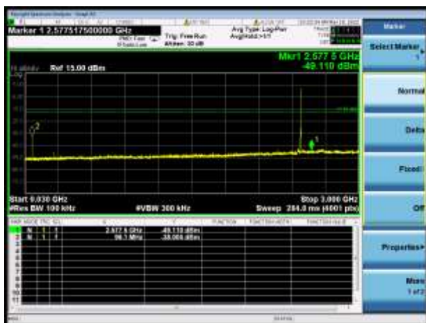
\pi/4 -DQPSK HIGH CHANNEL, SPURIOUS 30 MHz ~ 3 GHz
