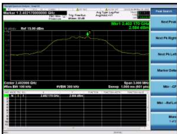
\pi/4 -DQPSK LOW CHANNEL, CARRIER LEVEL
